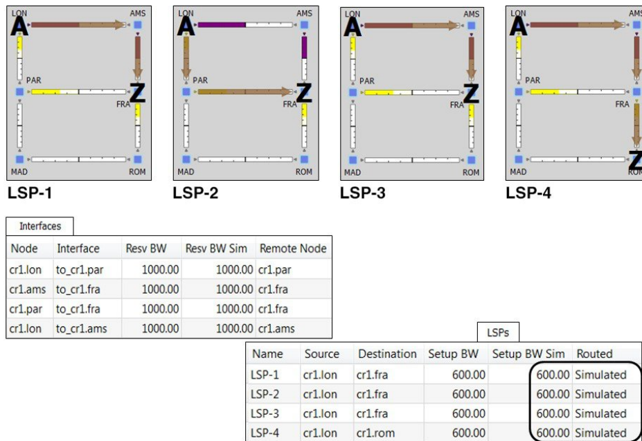
Figure 58: Simulated Routing Without Using Reservable Bandwidth Constraints
