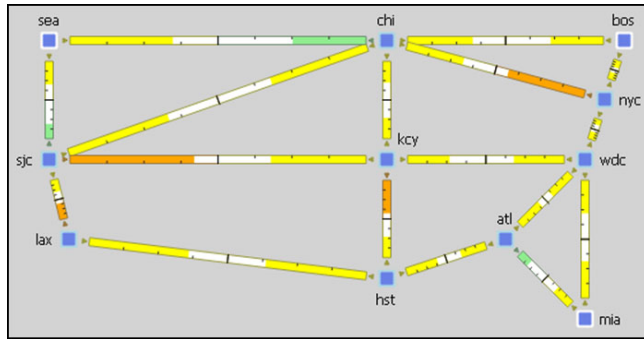
Figure 133: Network After Reducing Utilization to Below 90%
