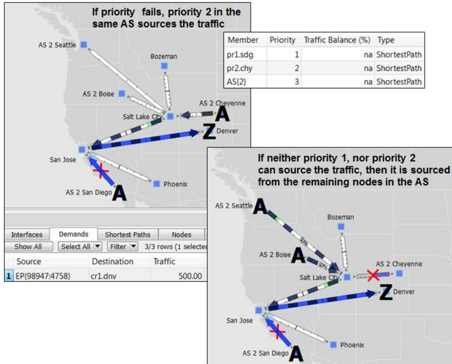
Figure 106: Example Failover Within the Same External AS
