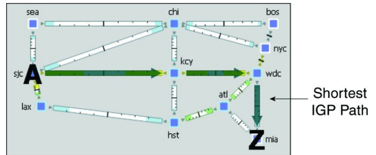
Figure 33: LSP Shortest IGP, Shortest TE, and Shortest Latency Paths
