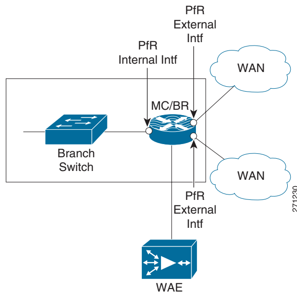
Figure 9-9 SOHO Deployment
