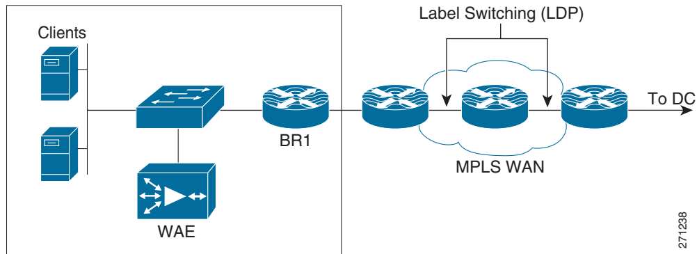
Figure 9-18 MPLS WAN
