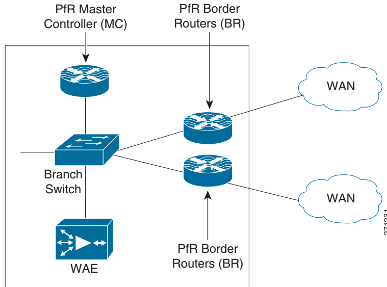
Figure 9-10 PfR Deployment with dual Branch Routers
