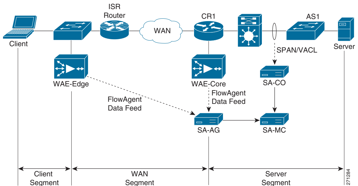
Figure 9-61 SuperAgent Distributed Configuration Example
