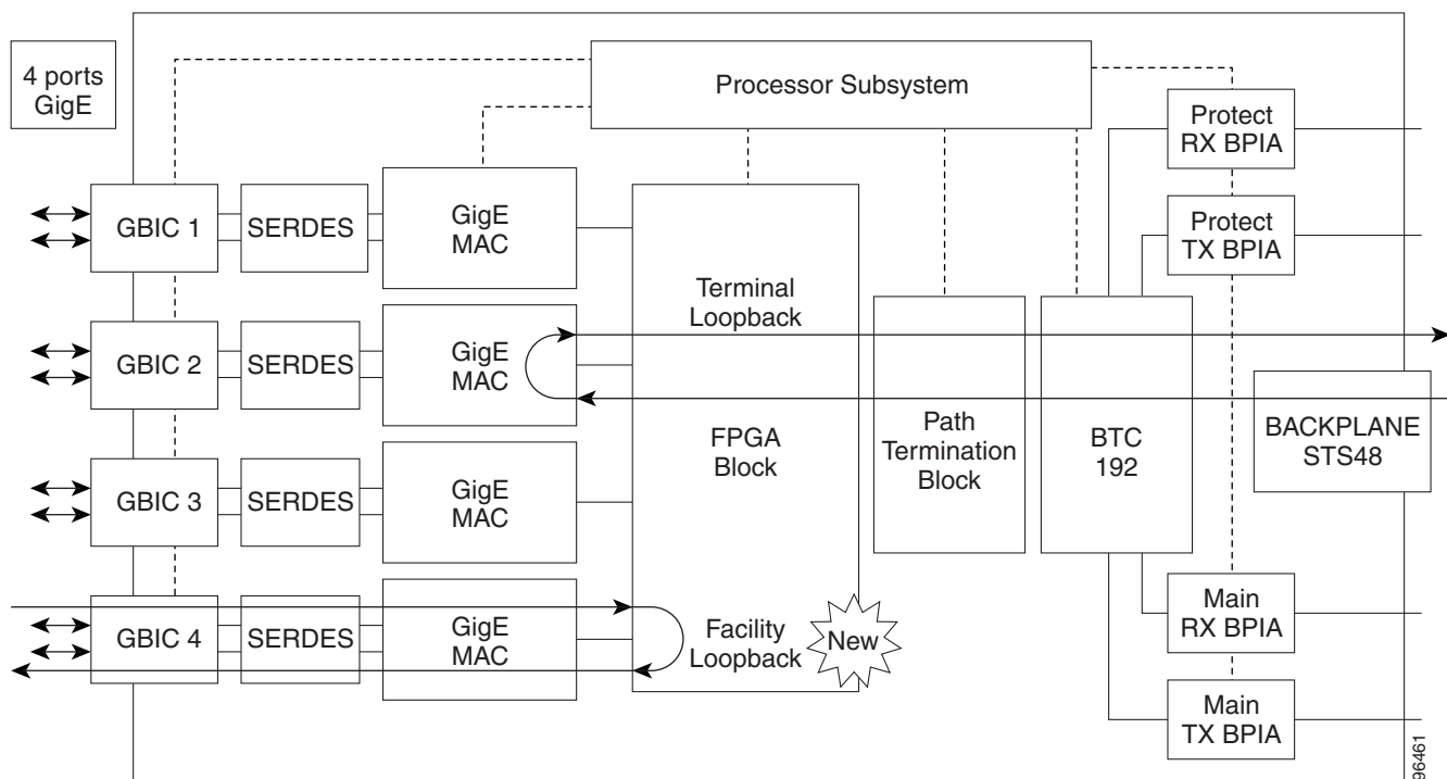
Figure 1-17 Terminal (Inward) Loopback on a G-Series Port
