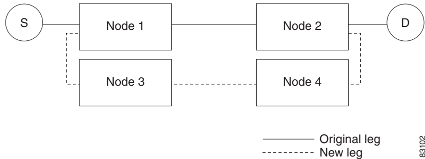
Figure 11-22 Dual Roll to Reroute to a Different Node
