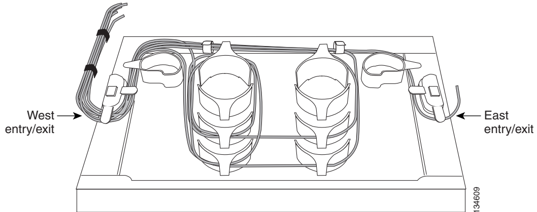
Figure 3-11 Fiber-Storage Tray
