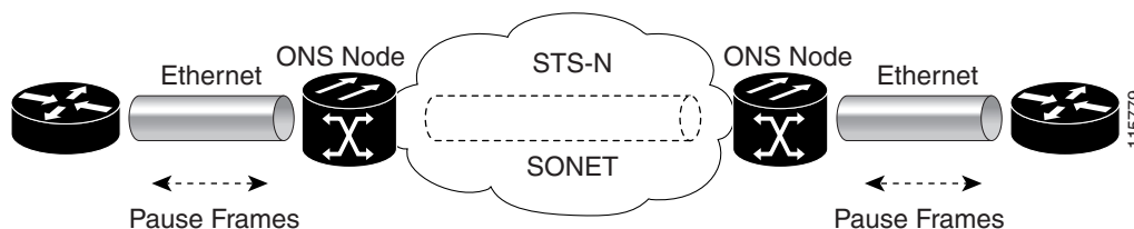
Figure 25-2 Flow Control
