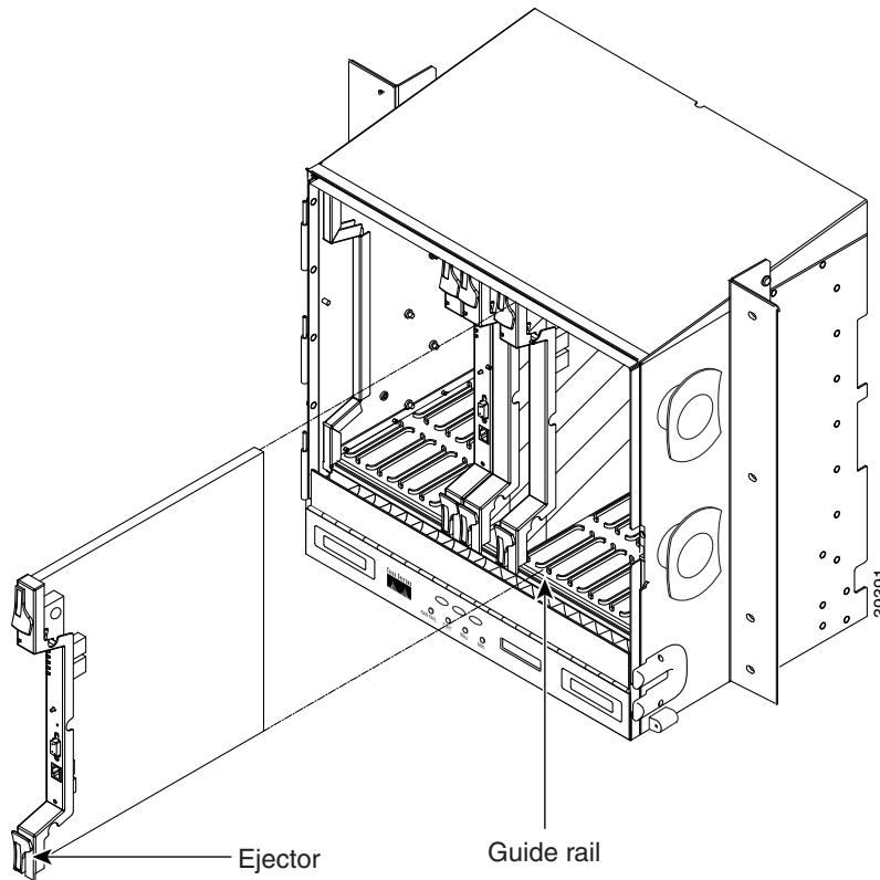
Figure 1-44 Installing Cards in the ONS 15454
