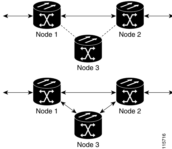
Figure 12-35 Unprotected Point-to-Point ADM to Path Protection Conversion
