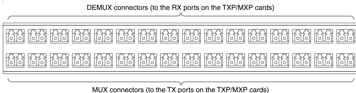
Figure 3-18 Front View of the Patch Panel
