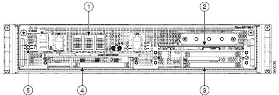
Figure 4: Cisco ASR 1002-X Router Slot Numbering
