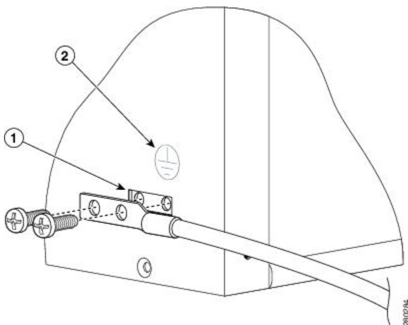
Figure 18: Attaching a Grounding Lug to the Chassis Ground Connector
