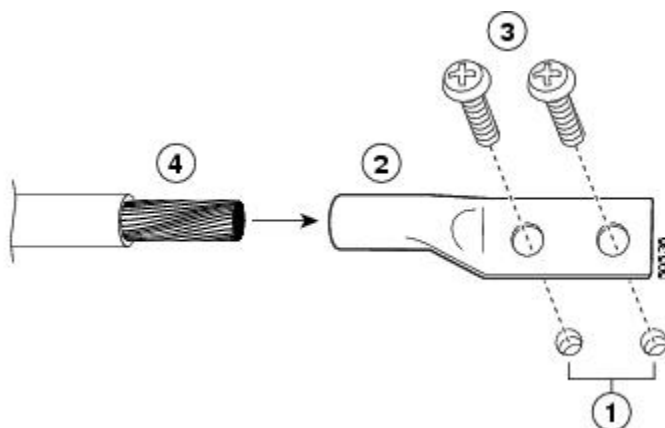
Figure 17: Parts of the Grounding Lug
