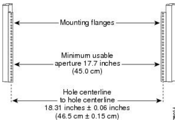
Figure 10: Verifying the Equipment Rack Dimensions
