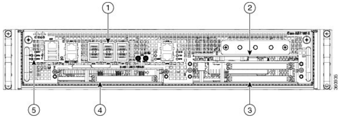
Figure 1: Cisco ASR 1002-X Router—Front View
