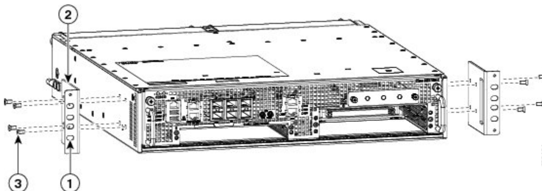
Figure 11: Attaching the Front Rack Mount Brackets to the Cisco ASR 1002-X Router
