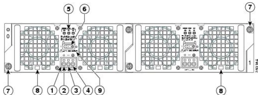
Figure 7: Cisco ASR 1002-X Router +24 VDC Power Supply
