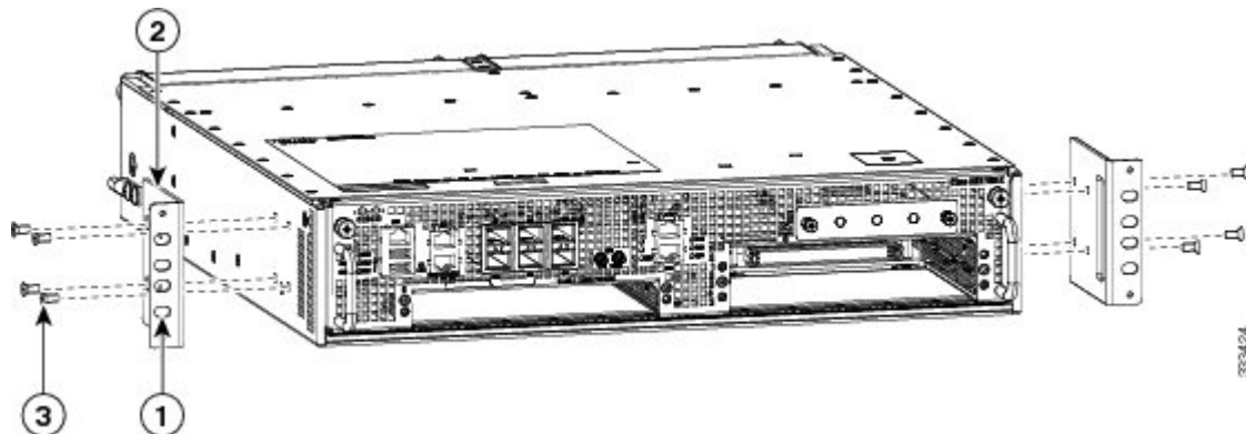
Figure 15: Chassis Rack Mount Bracket Ear Holes for the Cable Management Brackets
