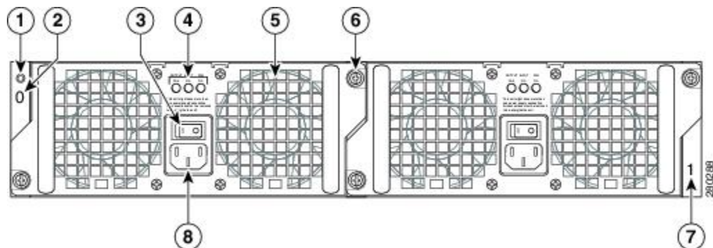
Figure 2: Cisco ASR 1002-X Router AC Power Supply
