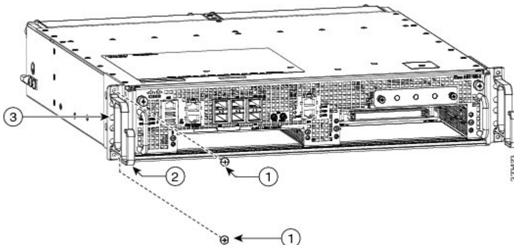
Figure 9: Attaching the Cable Management Brackets to the Cisco ASR 1002-X Router
