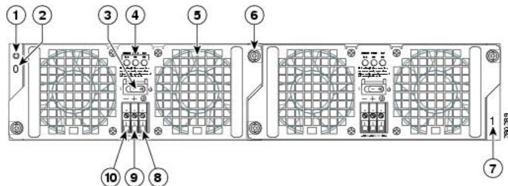
Figure 19: -48 VDC Power Supply for the Cisco ASR 1002-X Router
