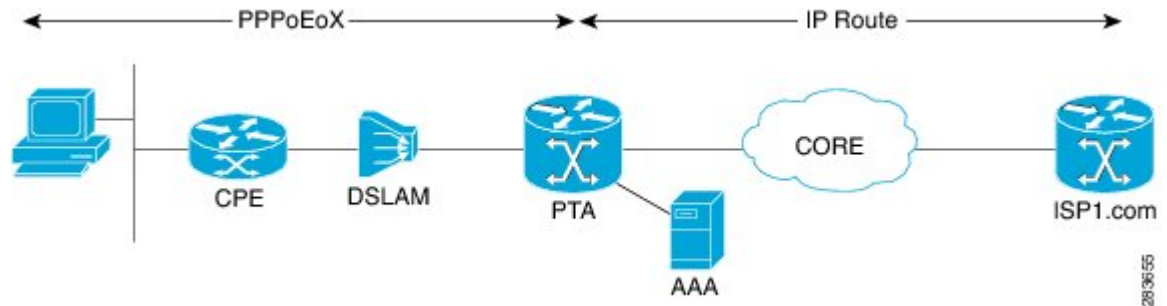
Figure 9: PPPoE-PTA Session
