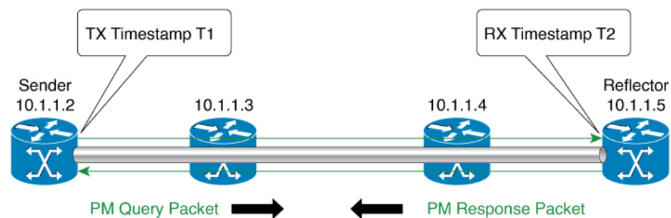
Figure 50: One-Way
