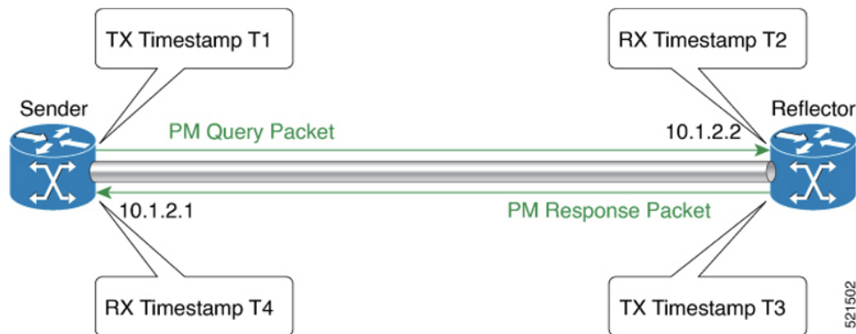
Figure 51: Two-Way
