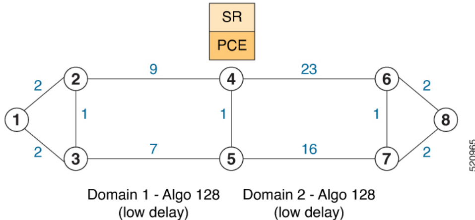
Figure 48: Multi-Domain Topology
