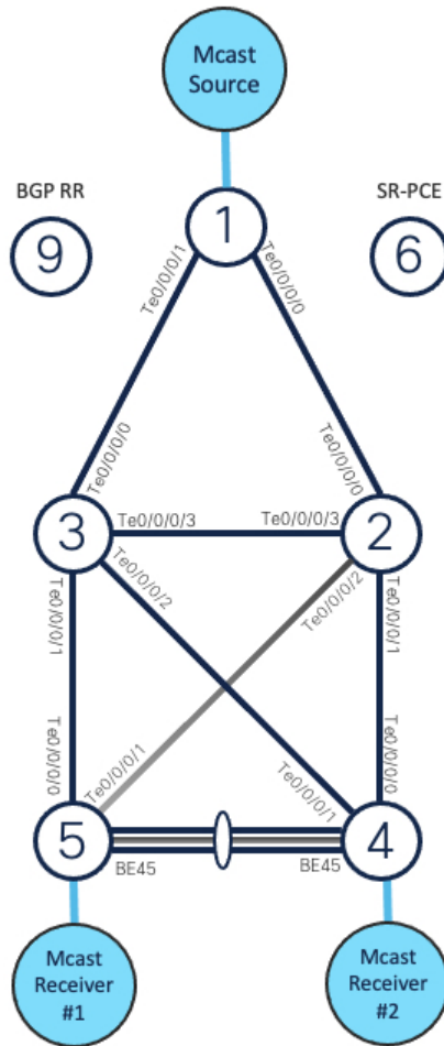
Figure 46: Topology
