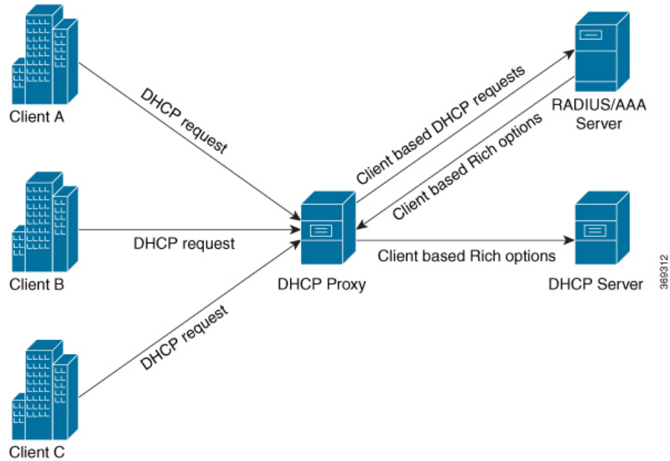
Figure 17: Flow of Rich Options From AAA Server to DHCP Proxy
