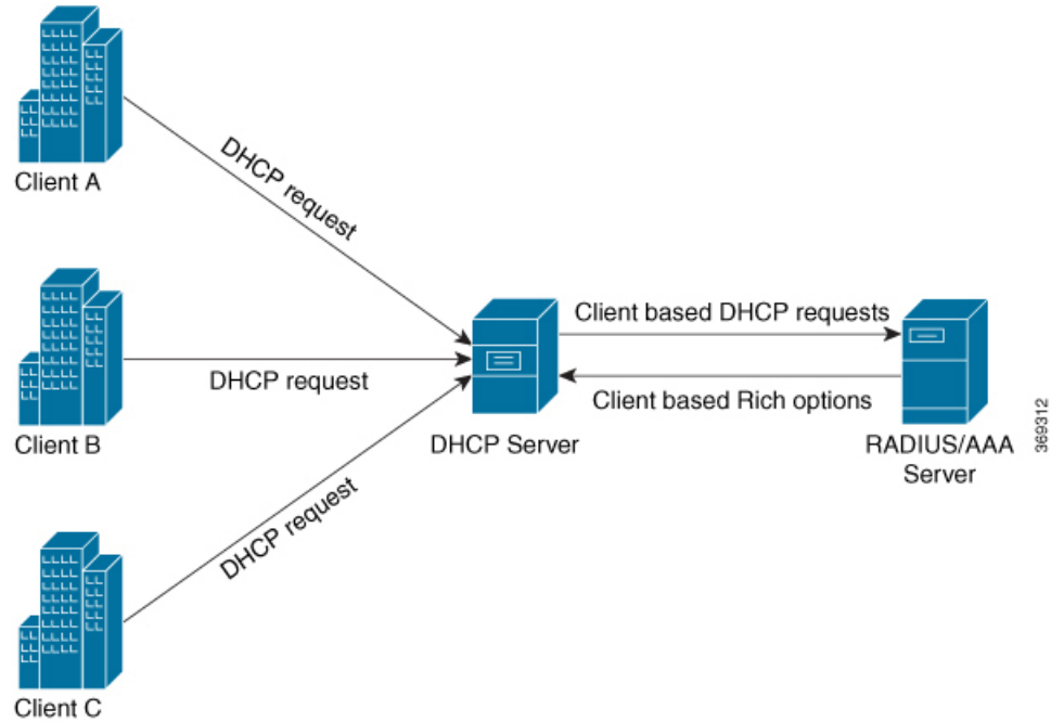
Figure 16: Flow of Rich Options From AAA Server to DHCP Server
