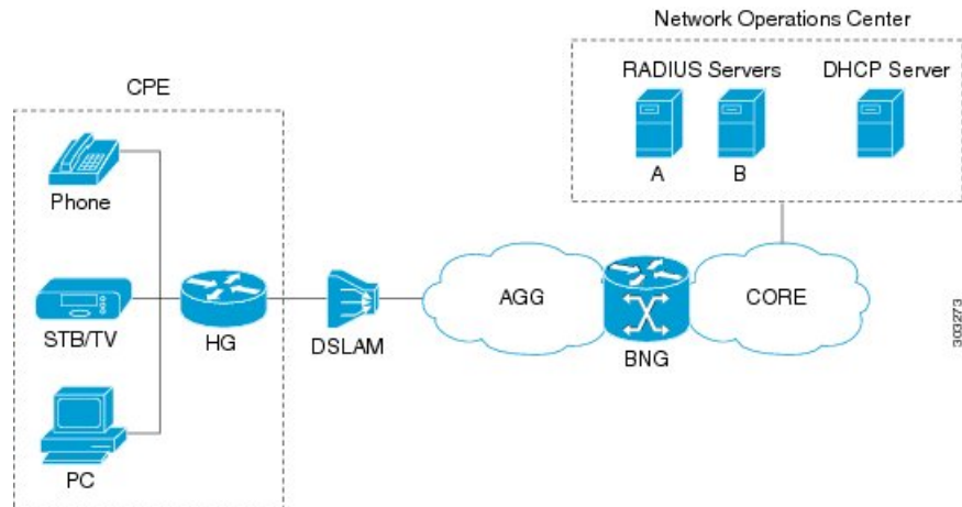
Figure 1: BNG Architecture
