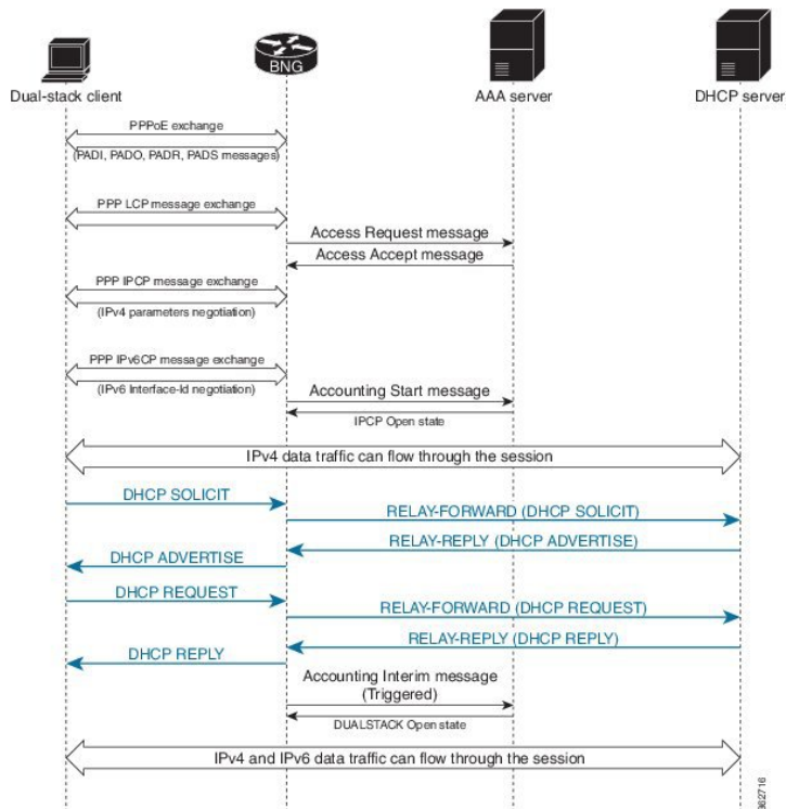
Figure 47: Call Flow of PPPoE Dual-Stack - DHCPv6-Based Address Assignment
