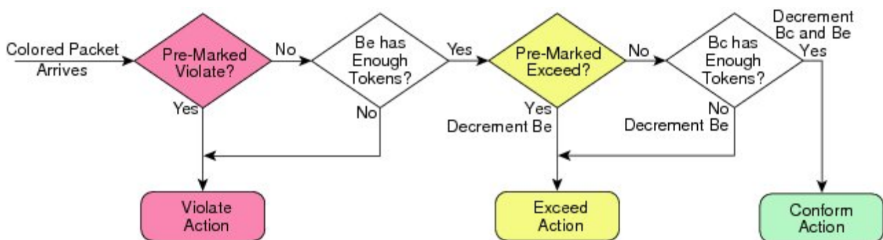
Figure 6: 2R3C Policing Process Flowchart
