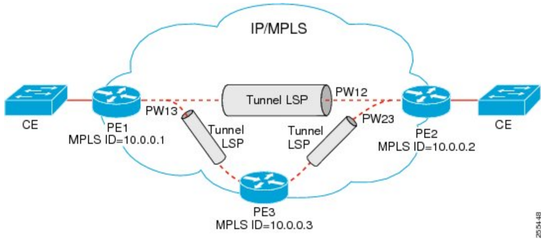
Figure 13: Typical VPLS Network Topology
