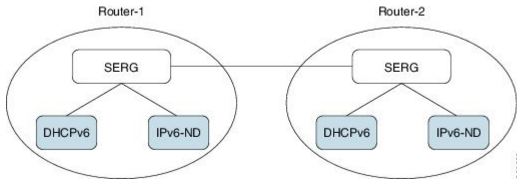
Figure 26: Geo Redundancy with a Single SERG
