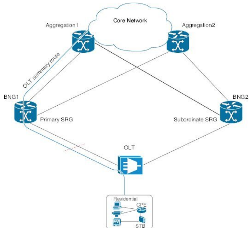
Figure 32: State Control Route for BNG Geo Redundancy
