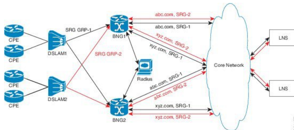
Figure 28: PPPoE-LAC Geo Redundancy Topology
