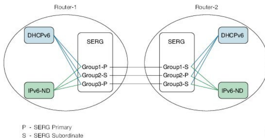
Figure 27: Geo Redundancy with Multiple SERGs
