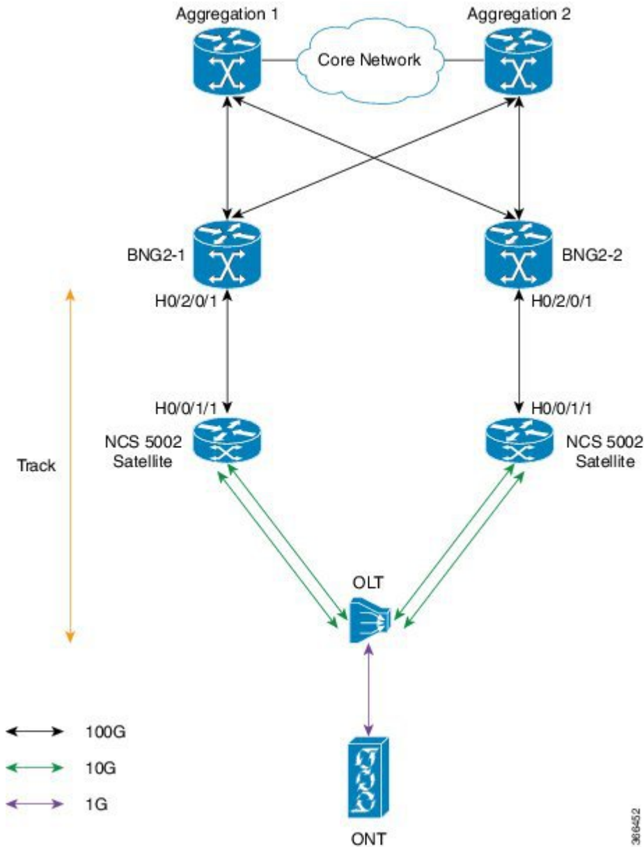
Figure 30: BNG Geo Redundancy with Cisco NCS 5000 Series nV Satellite
