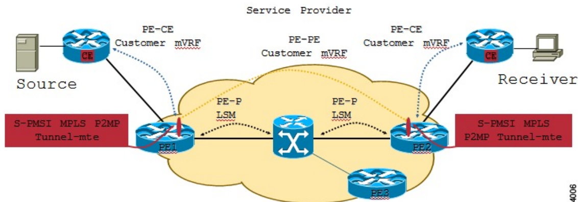
Figure 6: Multicast VRF
