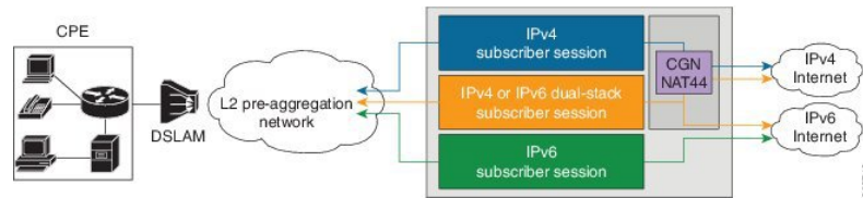
Figure 43: Deployment Model of Dual-Stack Subscriber Sessions
