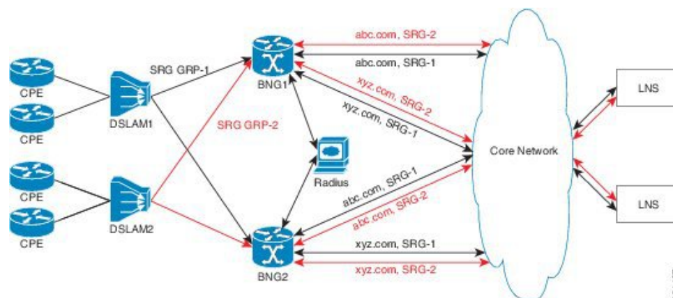
Figure 27: PPPoE-LAC Geo Redundancy Topology
