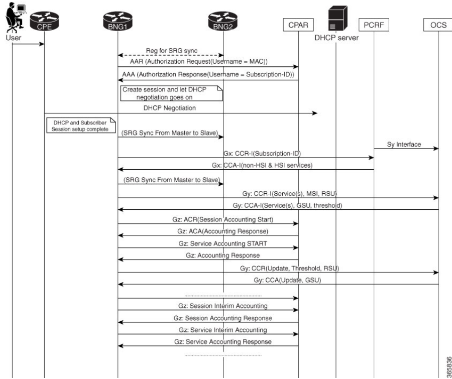
Figure 36: Call Flow of Subscriber Session Establishment With BNG DIAMETER-Geo Redundancy
