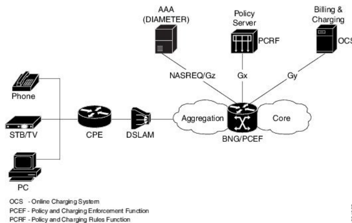
Figure 33: DIAMETER Interface in BNG
