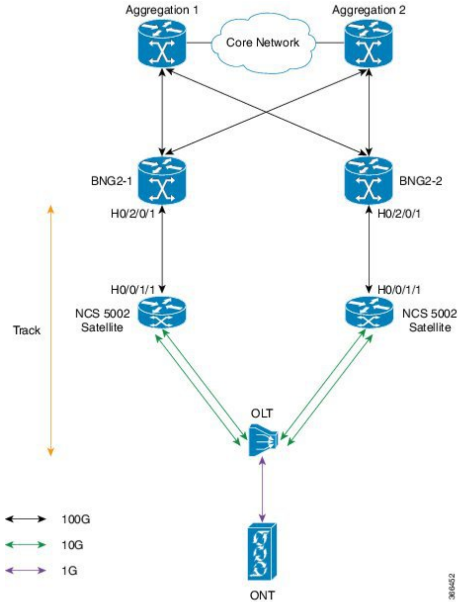
Figure 29: BNG Geo Redundancy with Cisco NCS 5000 Series nV Satellite
