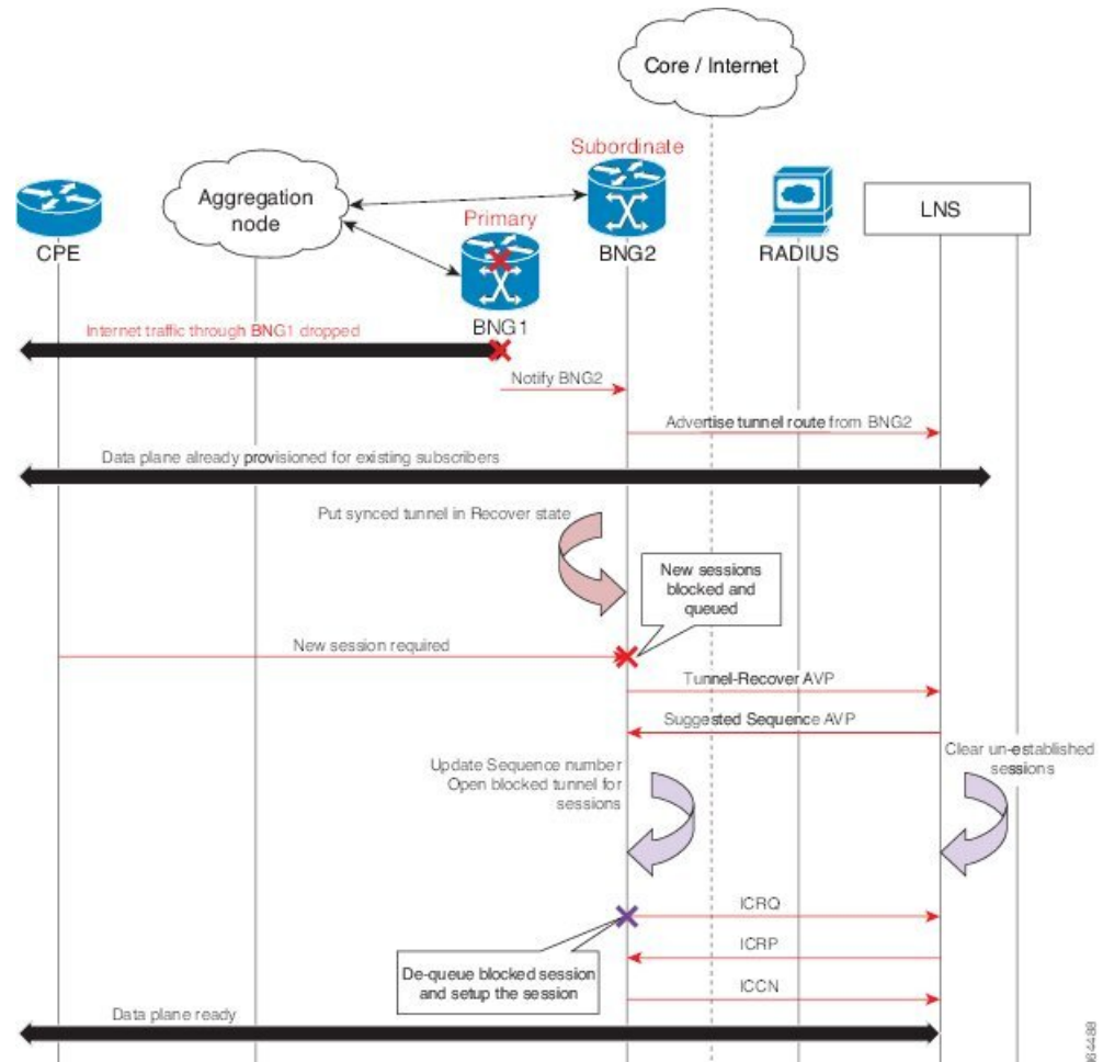
Figure 28: PPPoE-LAC Session Switchover
