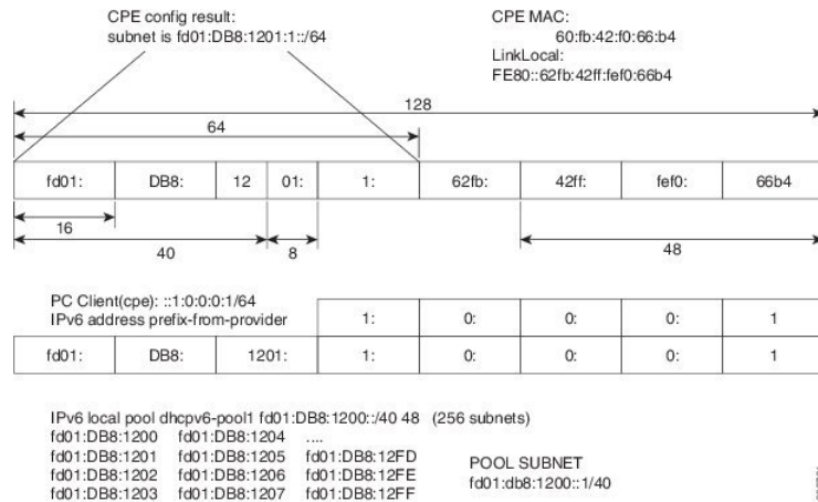
Figure 45: Sample IPv6 Address Mapping for Dual-Stack Subscriber
