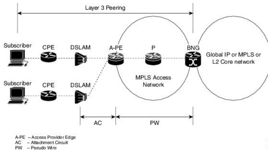
Figure 38: Sample Topology for BNG over Pseudowire Headend
