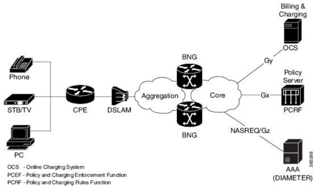
Figure 35: DIAMETER-Geo Redundancy Interworking
