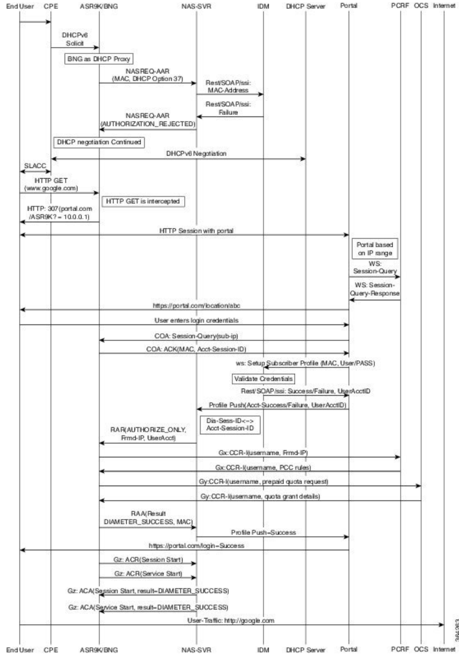
Figure 34: BNG DIAMETER Call Flow
