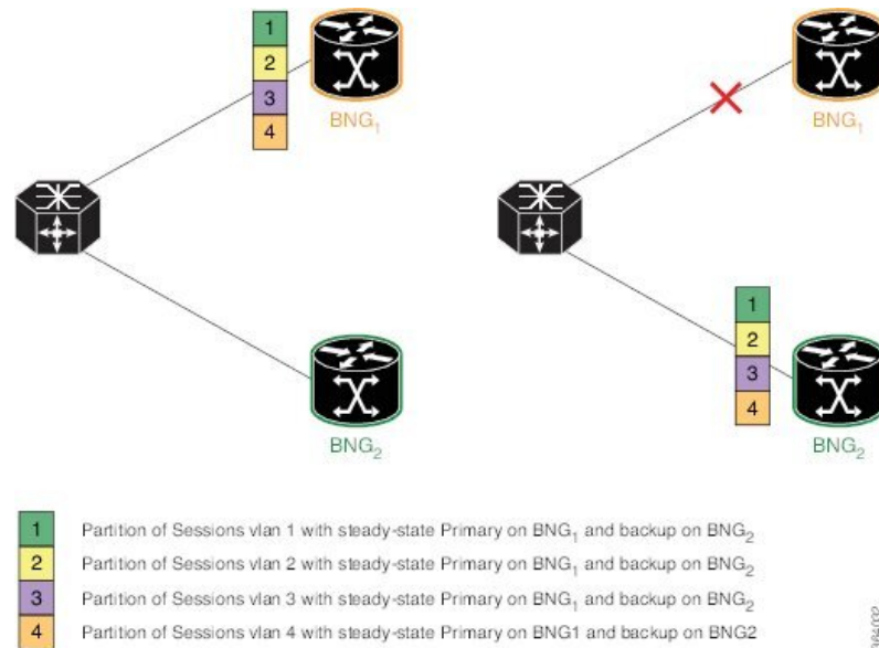
Figure 23: Active-standby Mode of Session Distribution
