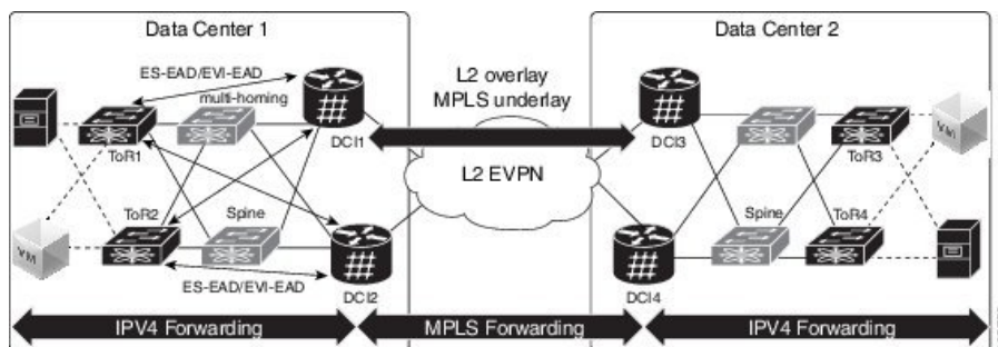
Figure 78: All-Active Multi Homing with Unique VTEP IP Address
