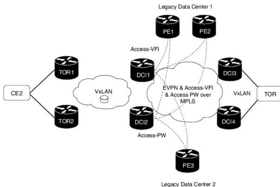
Figure 82: Virtual Ethernet Segment (vES)
