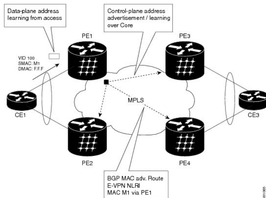
Figure 46: MAC Distribution in BGP (EVPN)
