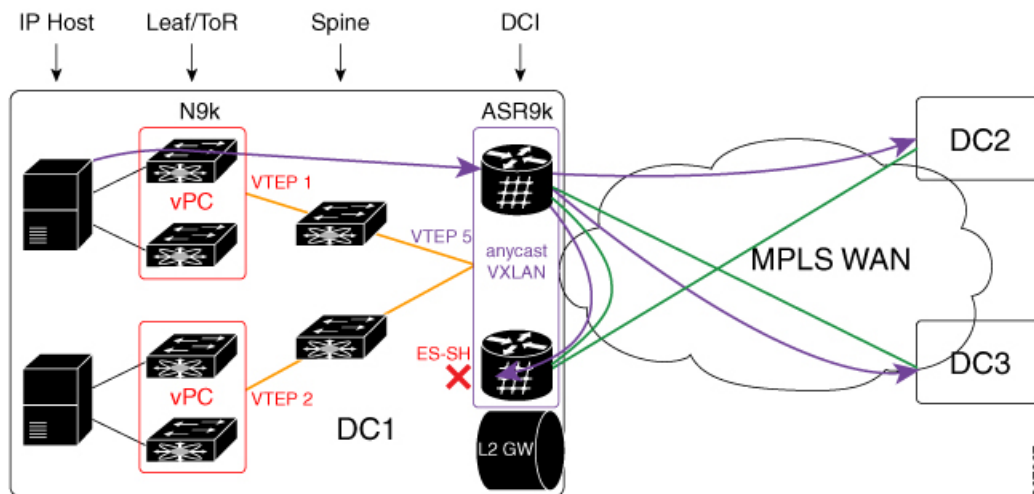
Figure 84: Anycast VXLAN L2 Gateway
