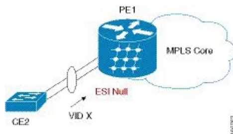
Figure 74: Single Home Device or Single Home Network (SHD/SHN)
