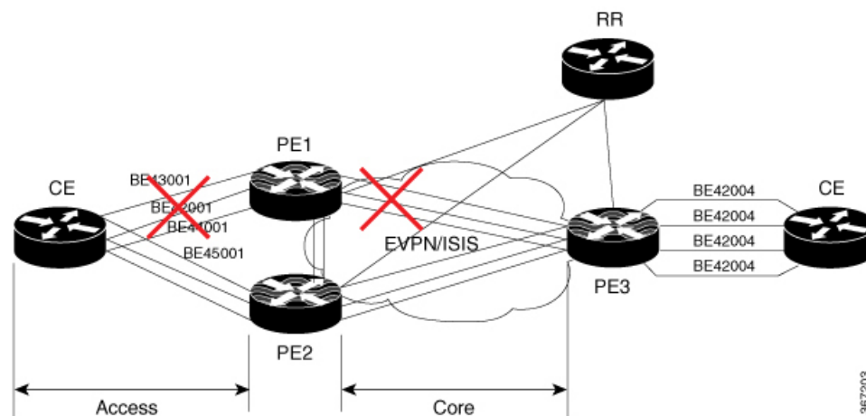
Figure 86: EVPN Core Isolation Protection
