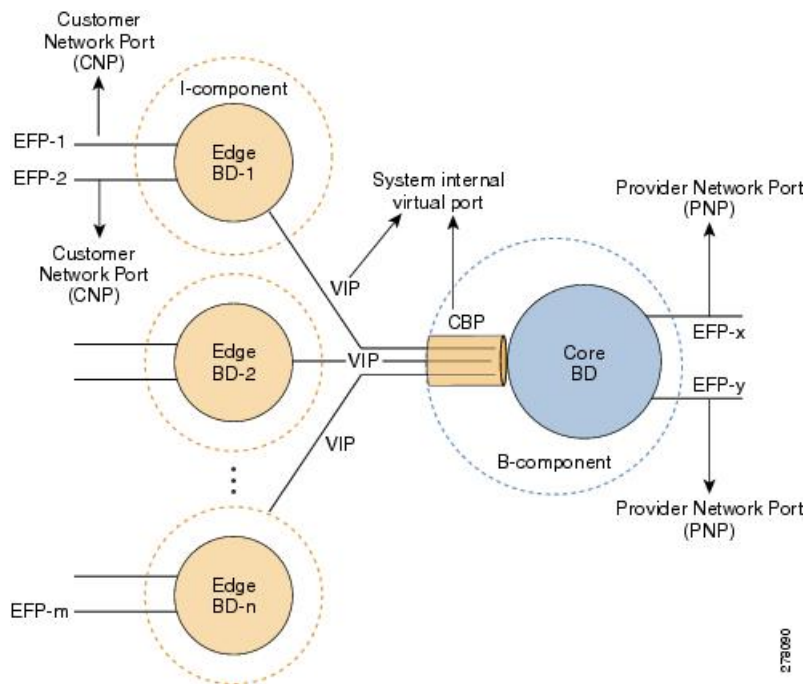
Figure 43: PBB Bridge Component Topology on Cisco ASR 9000 Series Routers
