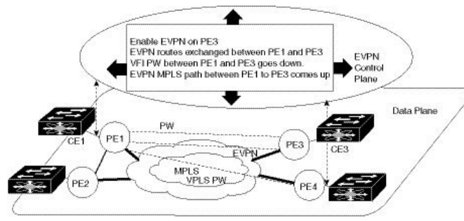
Figure 80: EVPN MPLS Seamless Integration with VPLS
