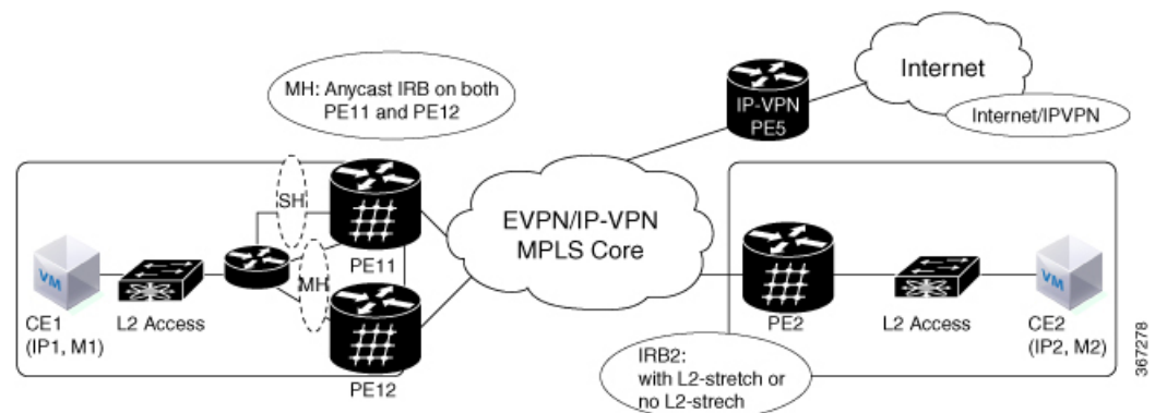
Figure 89: EVPN IRB with ASR 9000 as Centralized DCI Gateway
