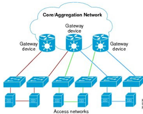
Figure 61: Access Networks
