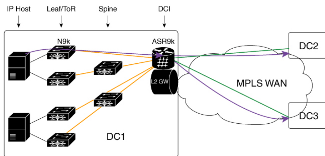
Figure 83: Single Homing VXLAN L2 GW
