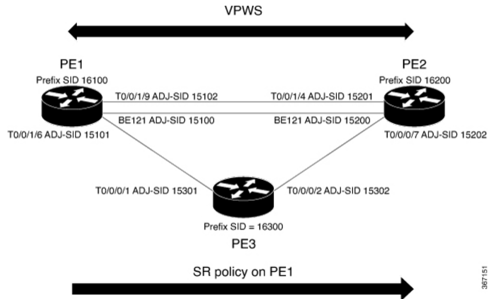
Figure 91: L2VPN VPWS and VPLS Preferred Path over SR-TE Policy
