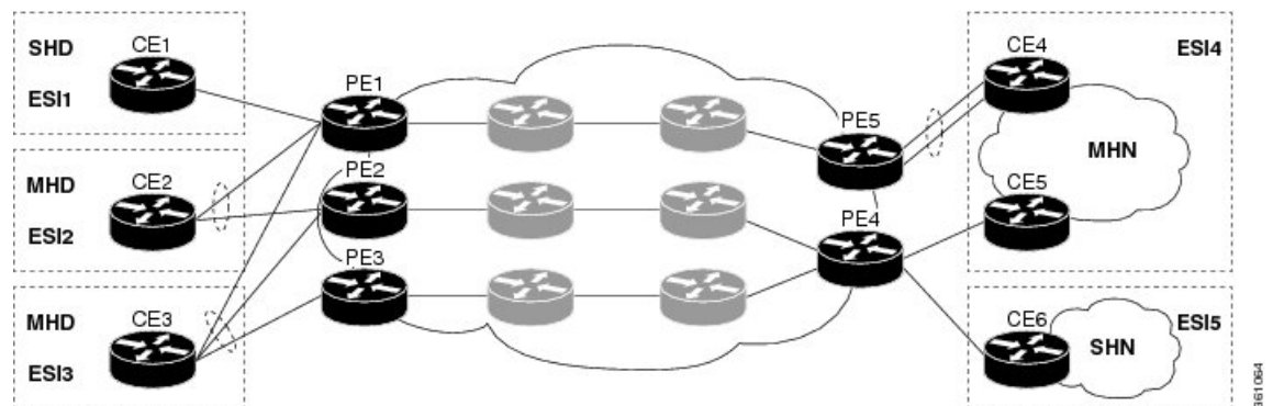
Figure 48: Ethernet Segment
