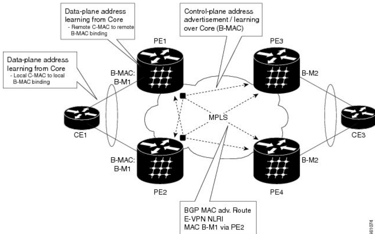
Figure 47: PBB-EVPN Network
