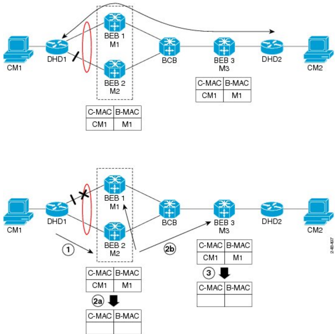
Figure 45: MIRP Operation
