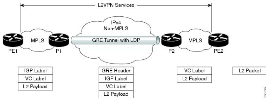
Figure 33: GRE tunnel configured between P to P routers
