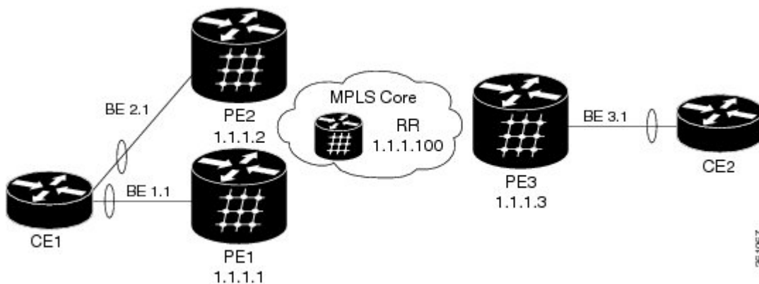
Figure 53: PBB EVPN on Dual Homed Device/Multi Homed Device with Active/Active per Service load-balancing and Dynamic Service Carving
