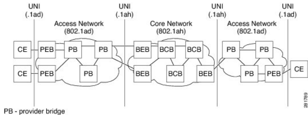
Figure 41: IEEE 802.1ah Provider Backbone Bridge
