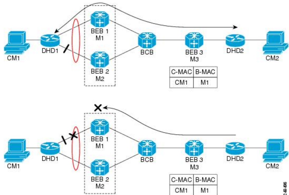
Figure 44: MIRP in 802.1ah Networks
