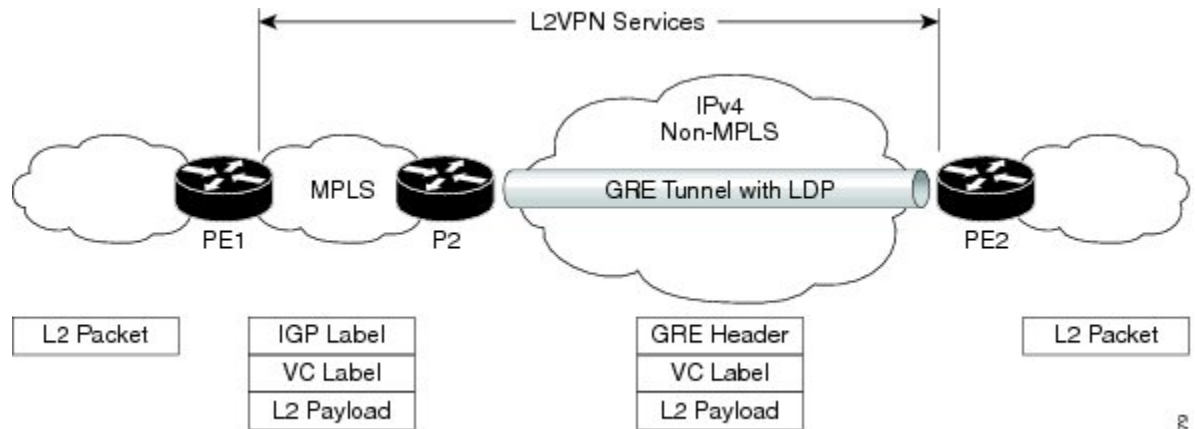
Figure 34: GRE tunnel configured between P to PE routers
