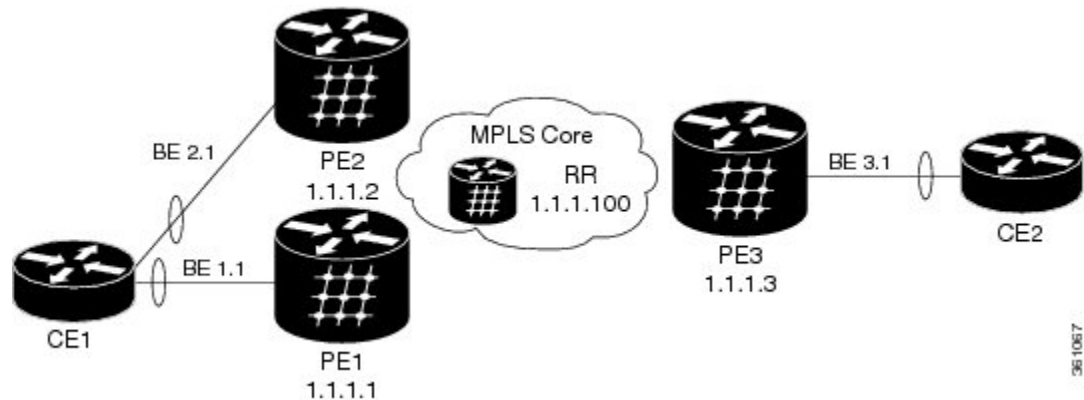
Figure 54: PBB EVPN on Dual Homed Device/Multi Homed Device with Active/Active per Service load-balancing and Manual Service Carving
