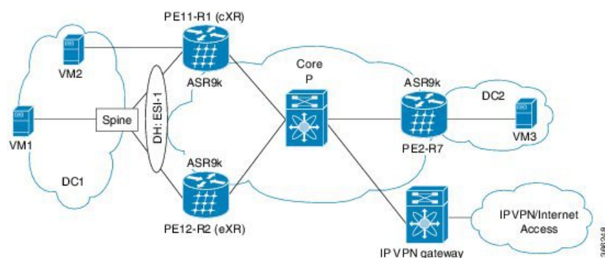
Figure 88: EVPN IRB
