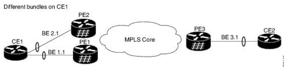
Figure 81: EVPN: Single-Active Multi-Homing
