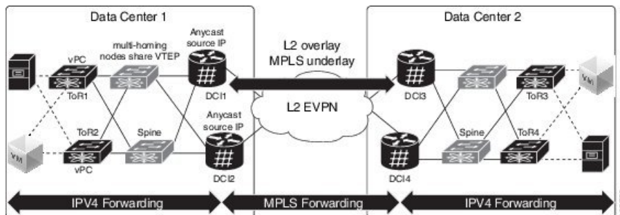
Figure 77: All-Active Multi Homing with Anycast VTEP IP Address
