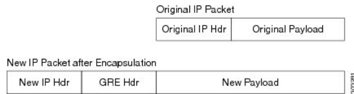
Figure 31: GRE Encapsulation
