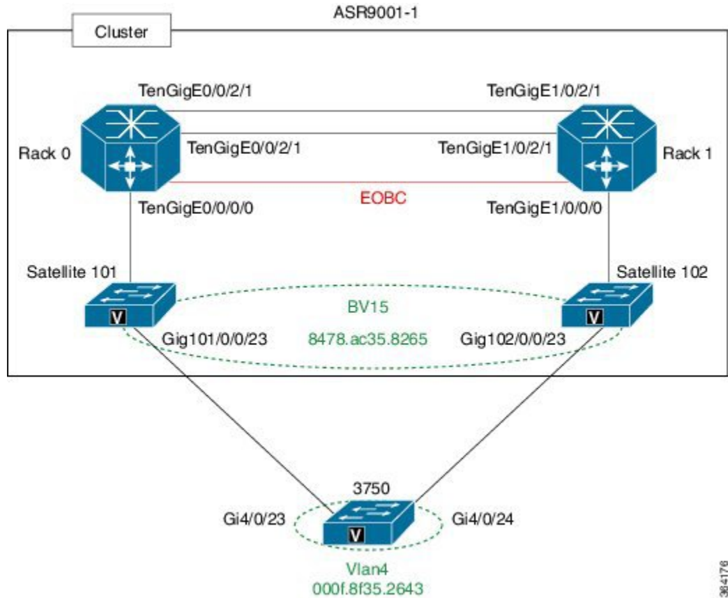
Figure 68: PVSTAG on a Cluster with a Satellite
