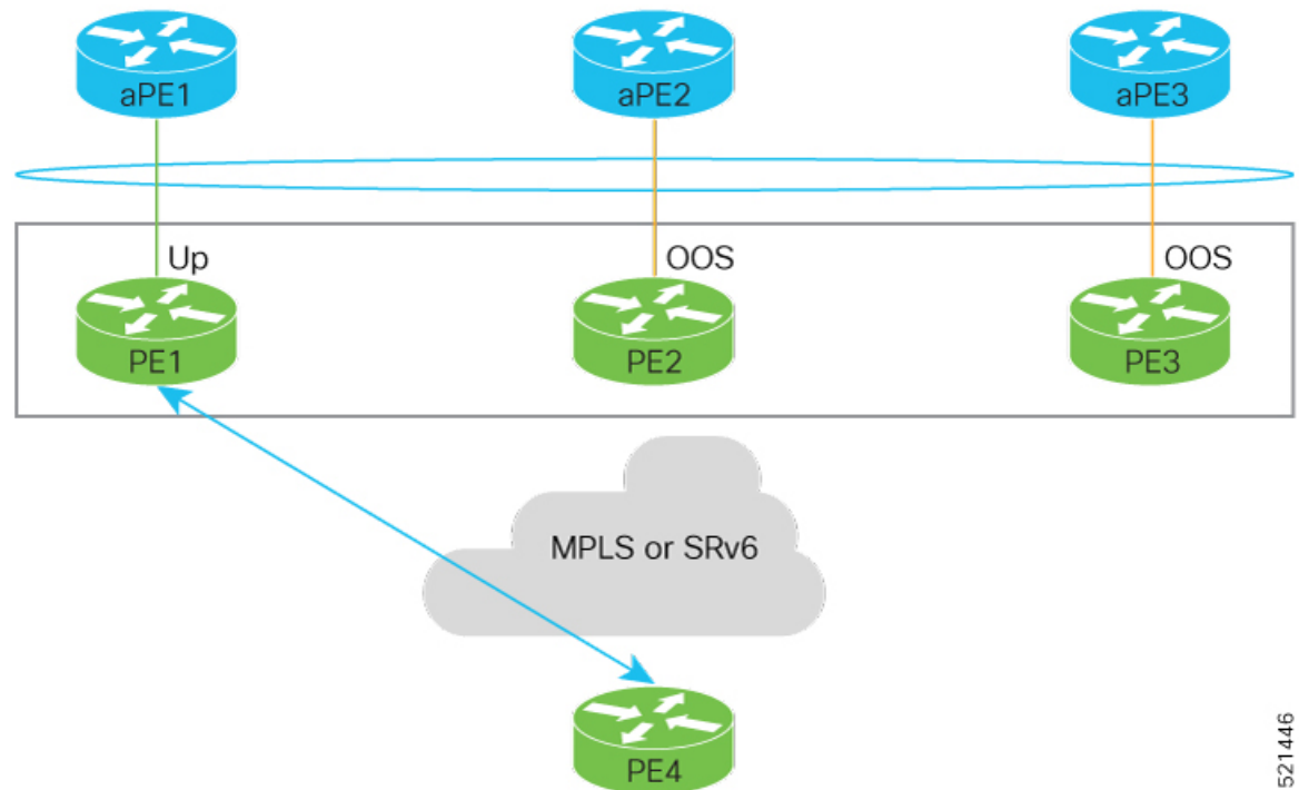
Figure 87: EVPN Access-Driven DF Election
