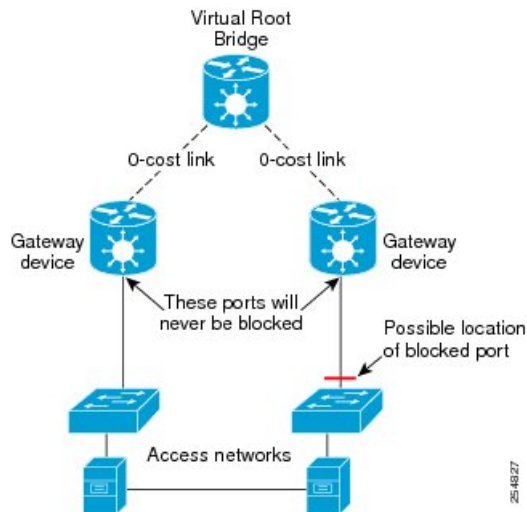
Figure 60: Access Network
