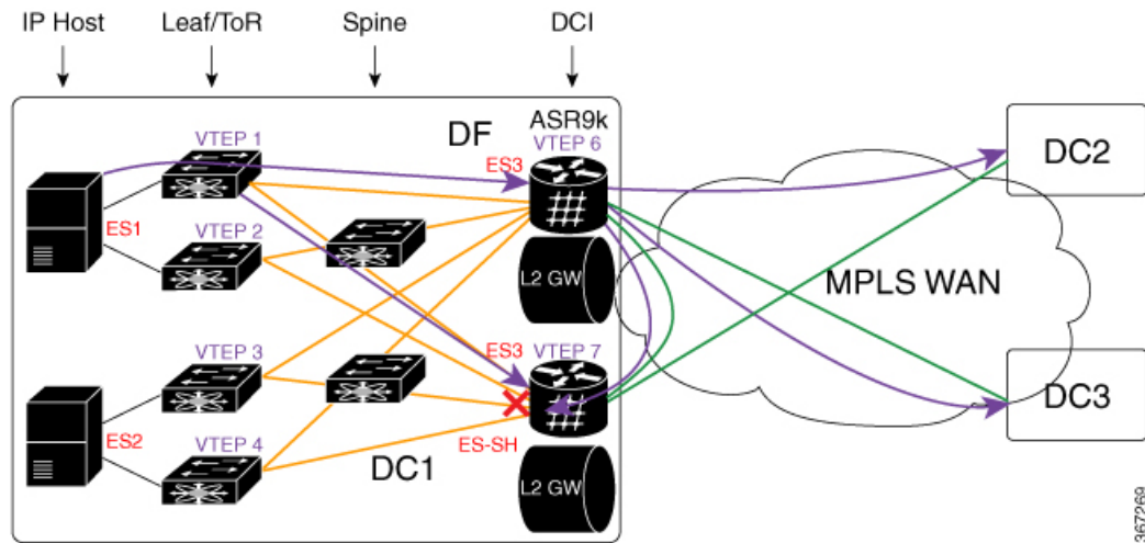
Figure 85: All-Active Multihoming VXLAN L2 Gateway
