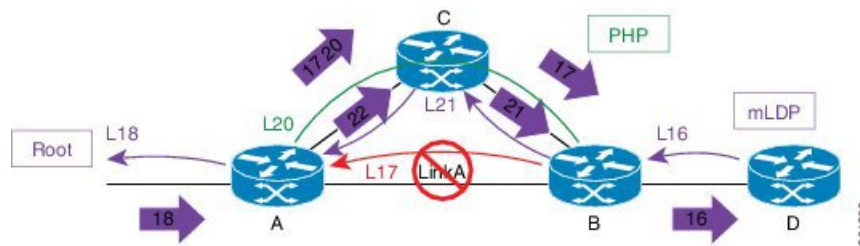
Figure 14: Re-optimization - Make-Before-Break
