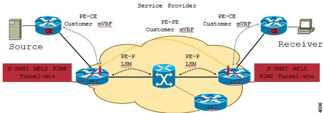
Figure 7: Multicast VRF
