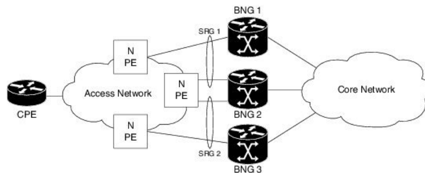
Figure 25: BNG Subscriber Redundancy Group
