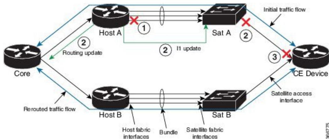
Figure 12: Host Side Detection of Active Links falling below the configured value
