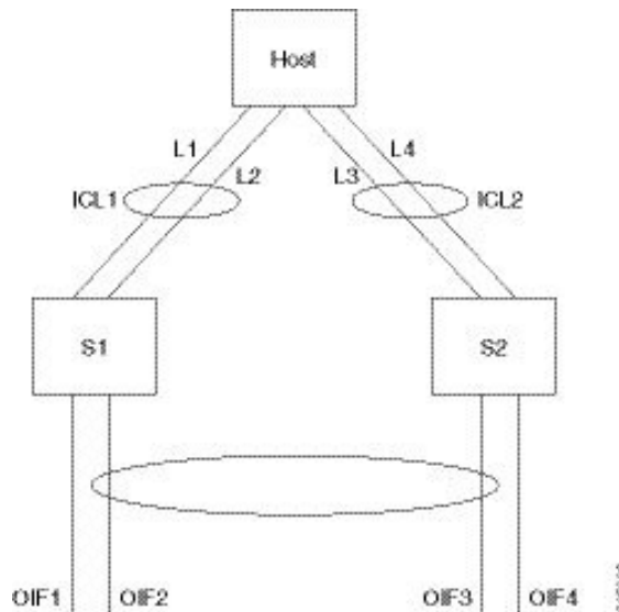
Figure 19: Multicast Offload Data Flow with ICL bundles to different satellites in Hub and Spoke topology
