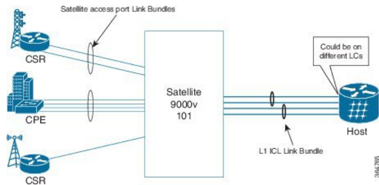
Figure 9: Multiple Access Bundles over many ICL bundles to Single Host
