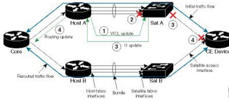
Figure 13: Satellite Side Detection of Active Links falling below the configured value
