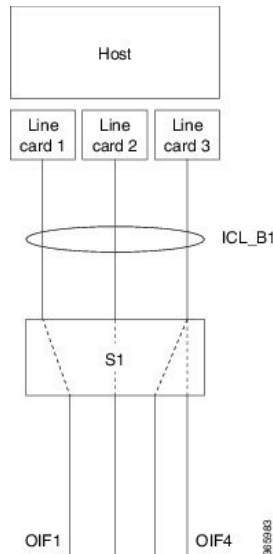
Figure 20: Multicast Offload with ICL bundle from different line cards to a satellite
