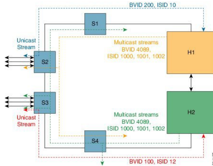
Figure 18: Multicast Offload Data Flow
