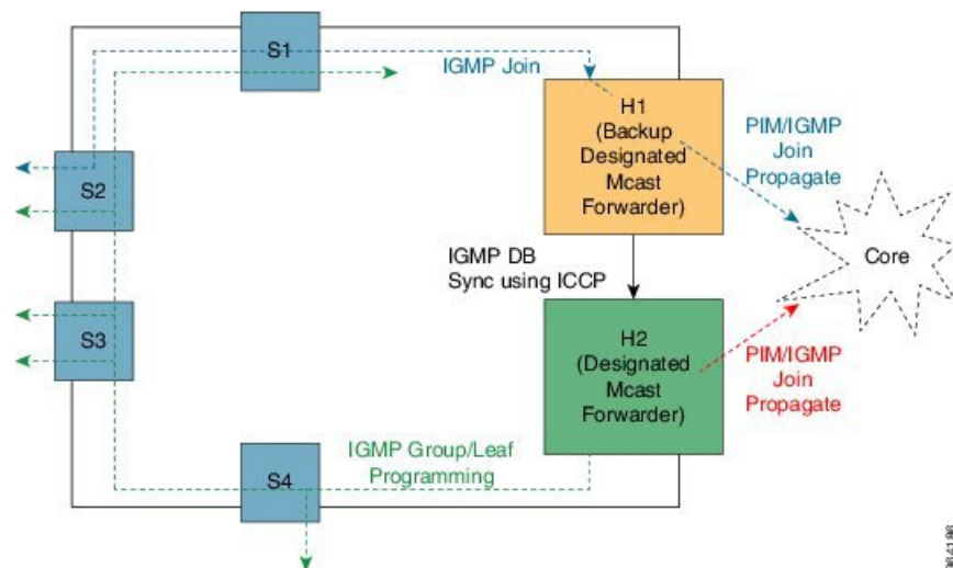
Figure 17: IGMP Join Programming (Access L2 and Core L2/BVI)
