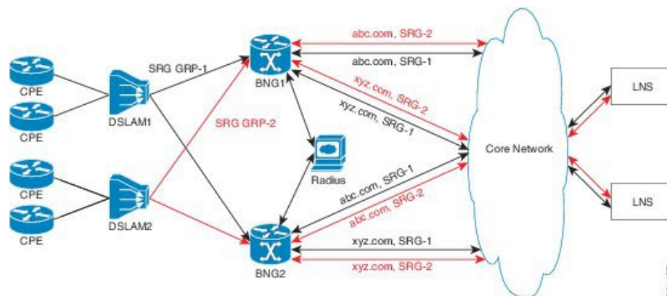
Figure 31: PPPoE-LAC Geo Redundancy Topology
