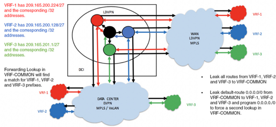
Figure 32: Inter-VRF Routing - Leak All Routes
