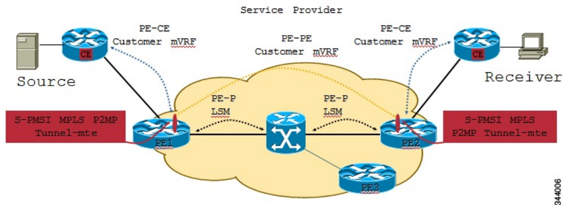
Figure 7: Multicast VRF
