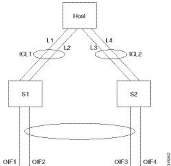
Figure 15: Multicast Offload Data Flow with ICL bundles to different satellites in Hub and Spoke topology
