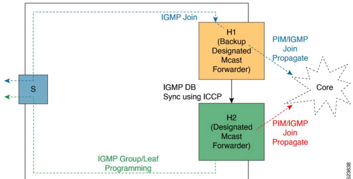
Figure 13: IGMP Join Programming (Access L2 and Core L2/BVI)
