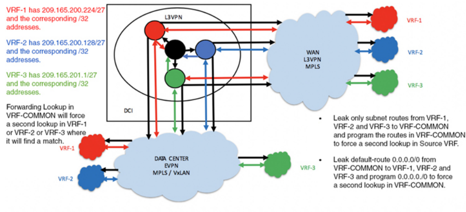
Figure 33: Inter-VRF Routing - Leak Only Subnet Routes
