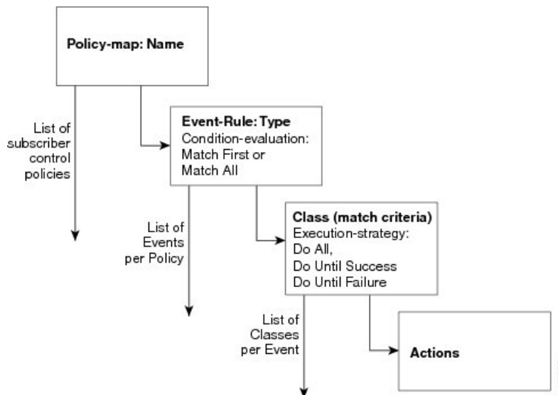
Figure 6: Control Policy
