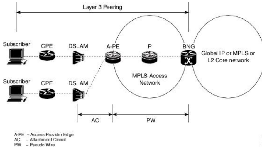
Figure 47: Sample Topology for BNG over Pseudowire Headend
