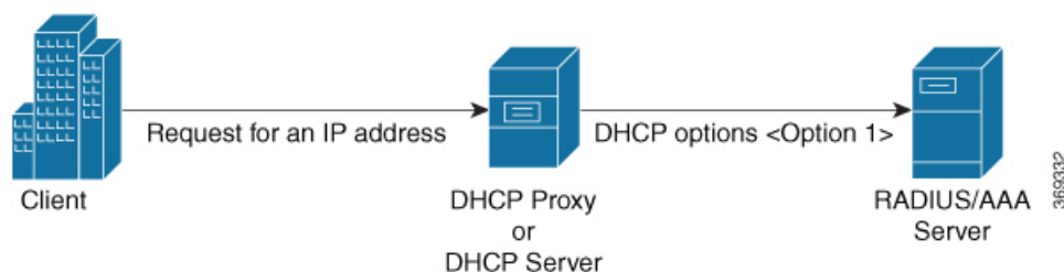
Figure 21: Flow of DHCP Options from DHCP Server or DHCP Proxy to the AAA Server
