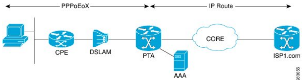
Figure 14: PTA Session
