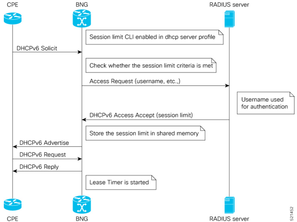
Figure 22: Sequence of events for limiting DHCPv6 sessions
