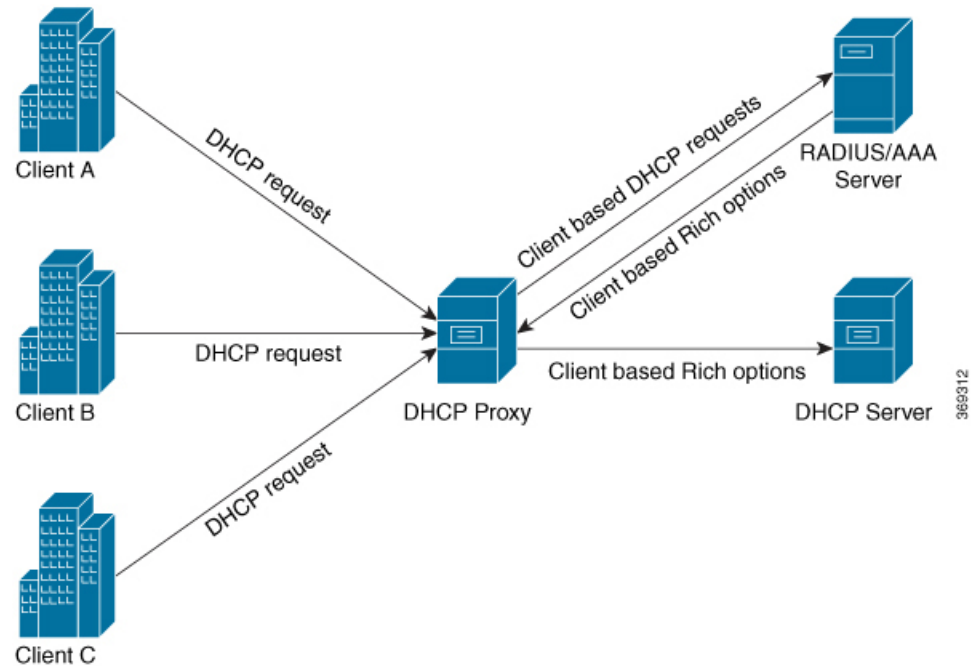
Figure 20: Flow of Rich Options From AAA Server to DHCP Proxy
