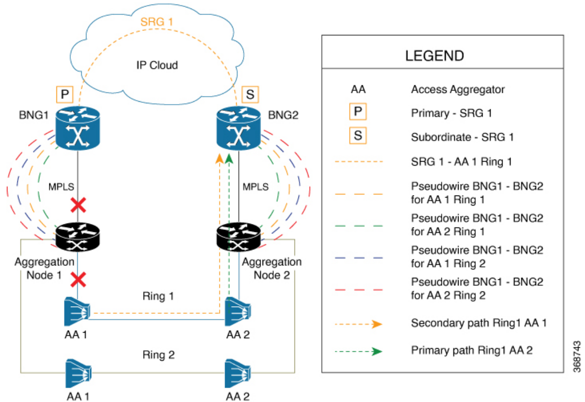
Figure 41: Link Failure Scenarios in BNG PWHE topology with SRG
