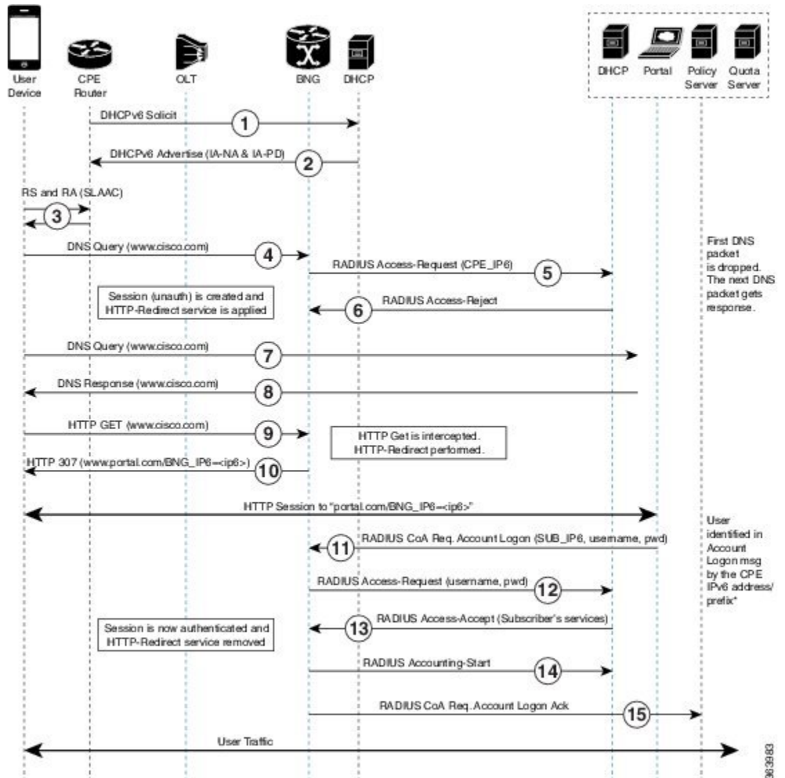
Figure 13: Call Flow of Web-logon IPv6 Routed Subscriber Session
