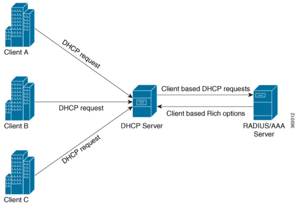
Figure 19: Flow of Rich Options From AAA Server to DHCP Server
