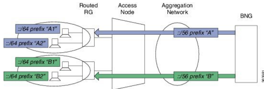
Figure 12: TR-177 Routed IPv6 Residential Gateway Deployment
