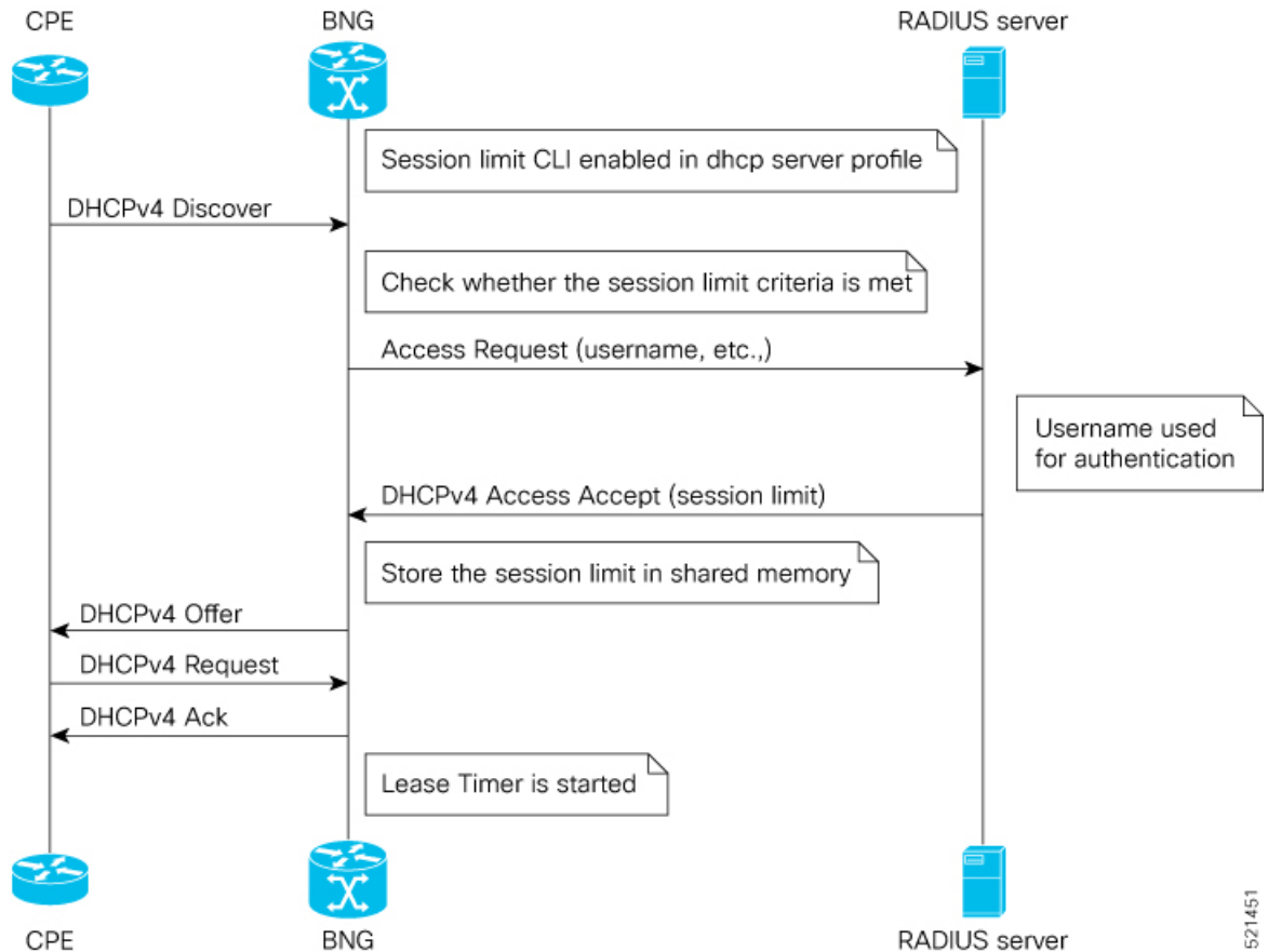
Figure 23: Sequence of events for limiting DHCPv4 sessions
