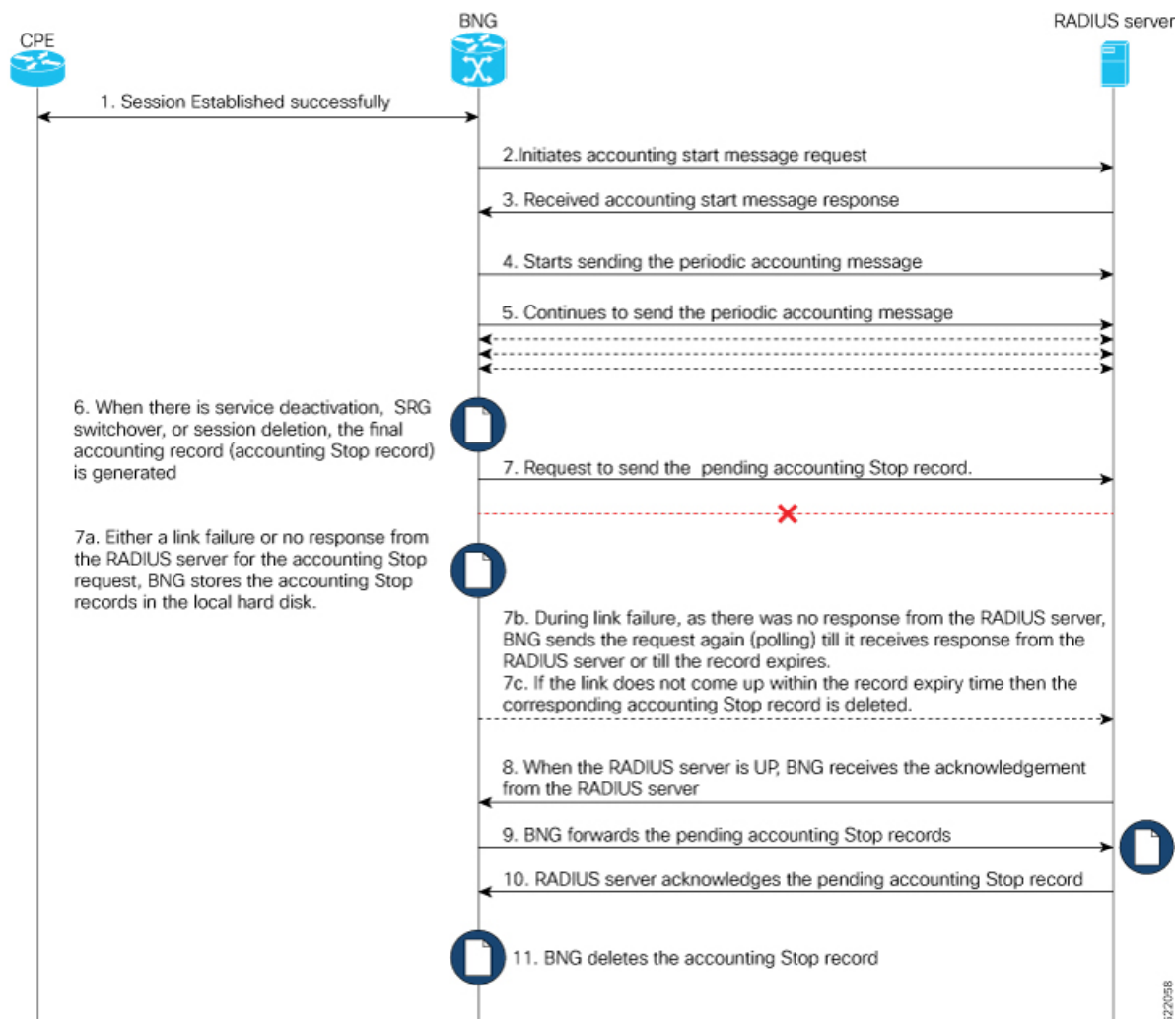
Figure 5: Sequence of events for forwarding accounting Stop record to the RADIUS Server
