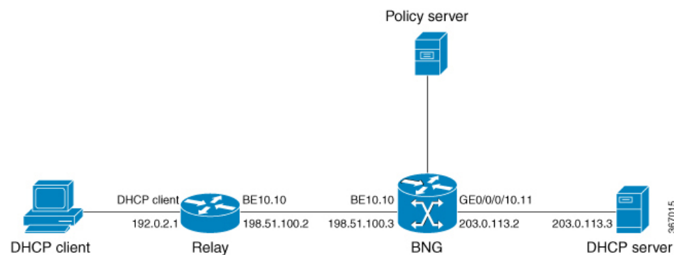
Figure 17: Network Topology of DHCP L3 Snooping in Cisco ASR 9000 BNG Router
