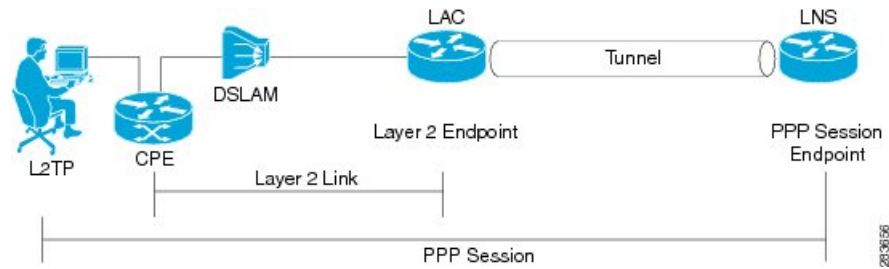
Figure 15: LAC Session
