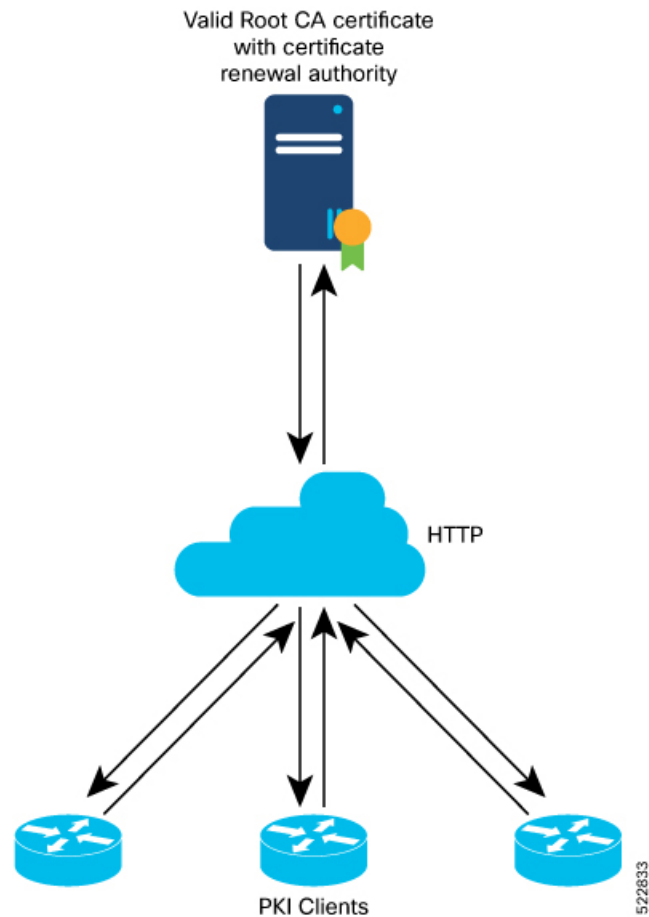
Figure 4: Automatic renewal of Public Key Infrastructure (PKI) certificate
