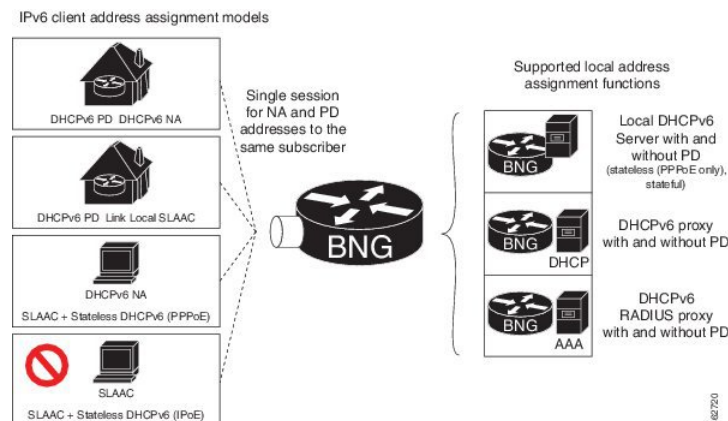
Figure 53: IPv6 Client Address Assignment Models
