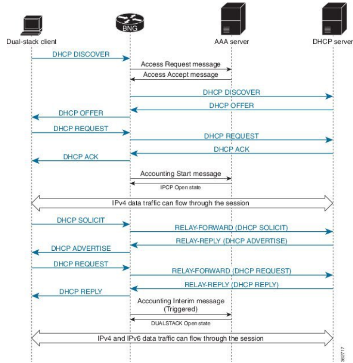
Figure 58: Call Flow of IPoE Dual-Stack - IPv4 Address-Family Starts First
