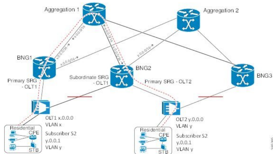
Figure 39: Peer-to-peer Traffic Flow with BNG Geo Redundancy
