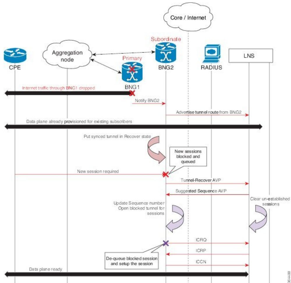
Figure 35: PPPoE-LAC Session Switchover
