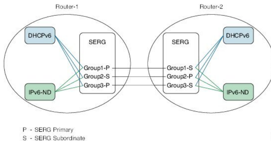
Figure 33: Geo Redundancy with Multiple SERGs
