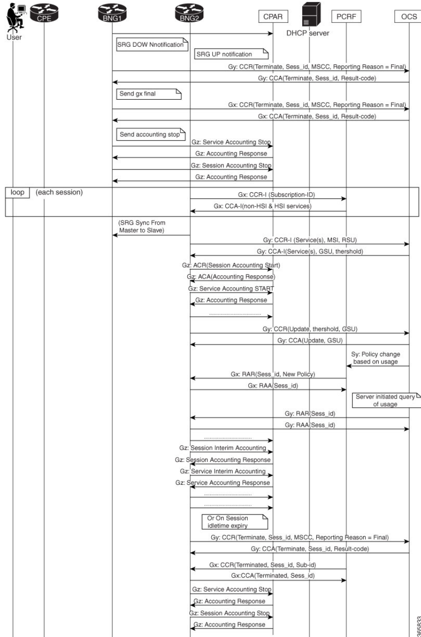
Figure 46: Call Flow of Subscriber Sessions During SRG Switch Over
