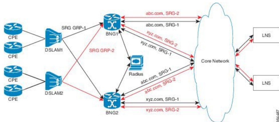
Figure 34: PPPoE-LAC Geo Redundancy Topology
