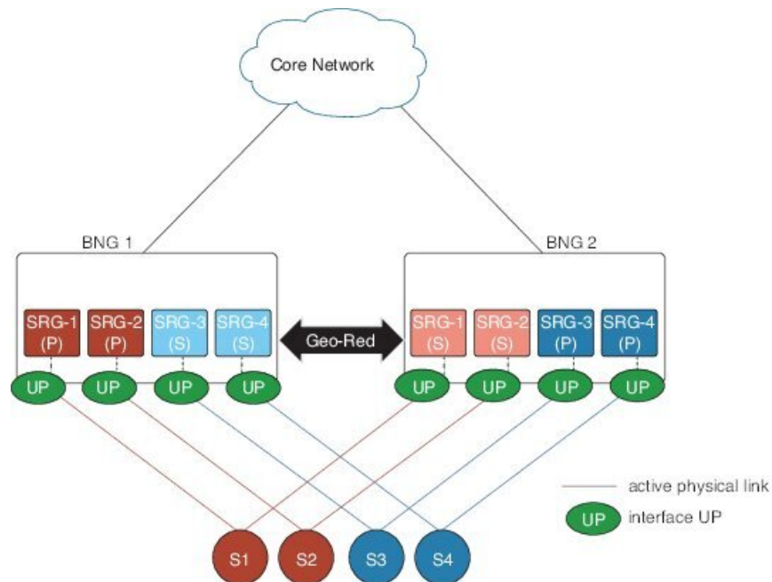
Figure 37: Active-active Session for BNG Geo Redundancy
