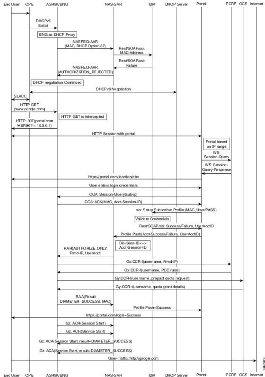
Figure 43: BNG DIAMETER Call Flow
