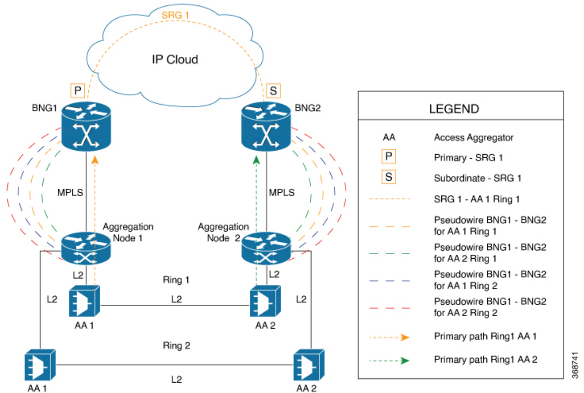
Figure 40: Sample Network Topology of SRG for PWHE Subscriber Sessions on BNG
