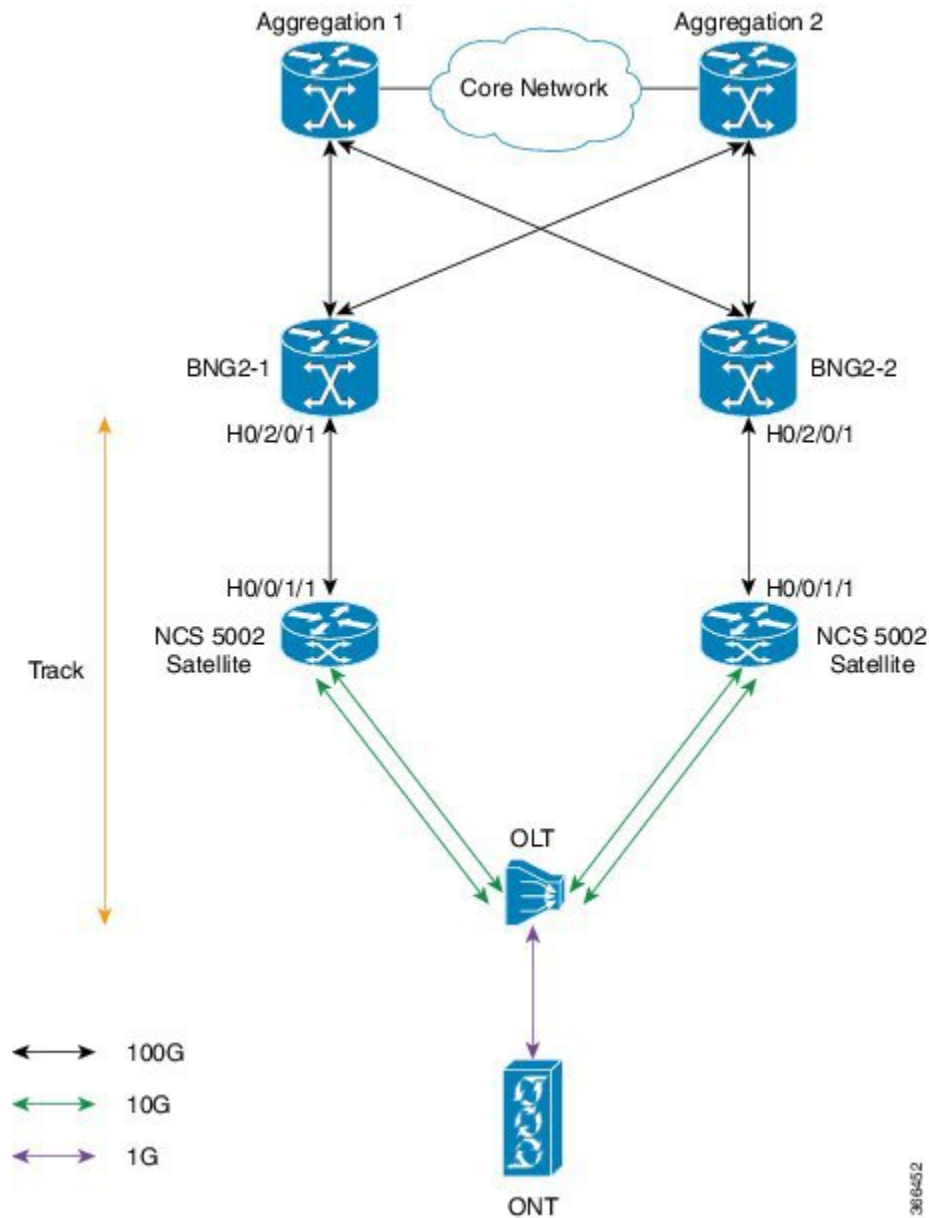
Figure 36: BNG Geo Redundancy with Cisco NCS 5000 Series nV Satellite
