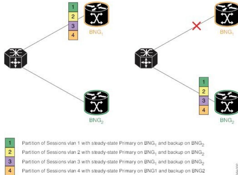
Figure 30: Active-standby Mode of Session Distribution
