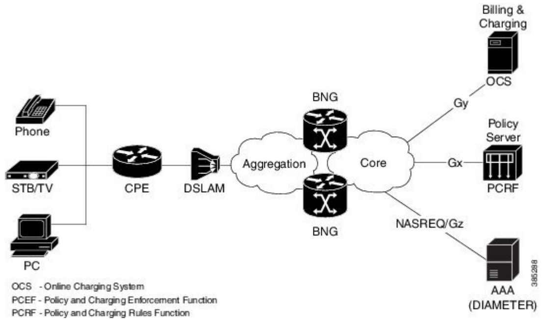
Figure 44: DIAMETER-Geo Redundancy Interworking
