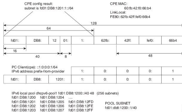
Figure 54: Sample IPv6 Address Mapping for Dual-Stack Subscriber
