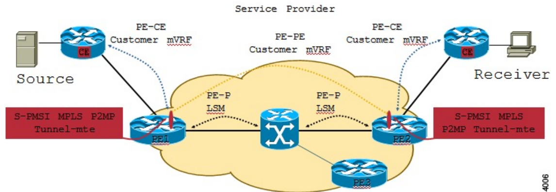
Figure 7: Multicast VRF
