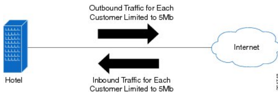
Figure 16: Bidirectional UBRL scenario
