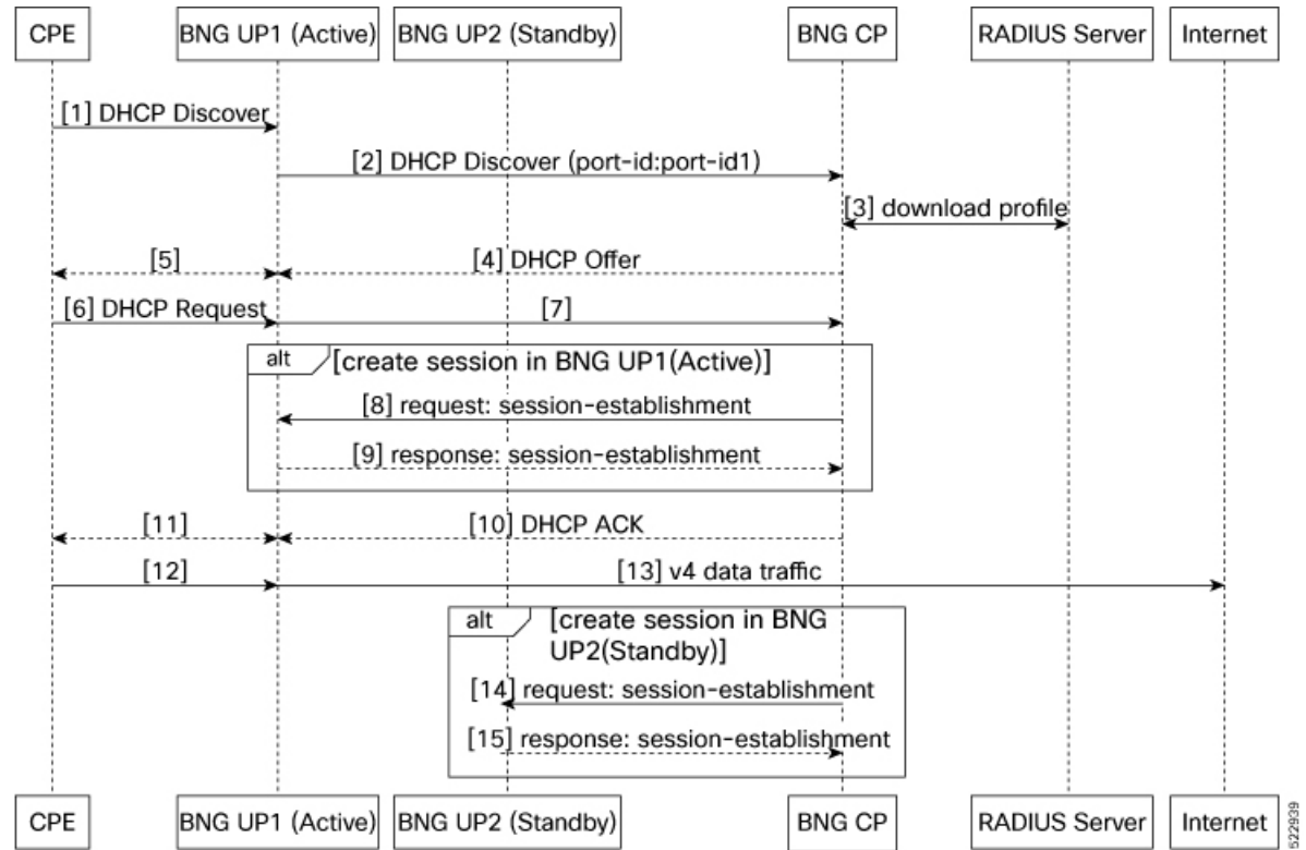
Figure 10: Subscriber Session Creation for SRG
