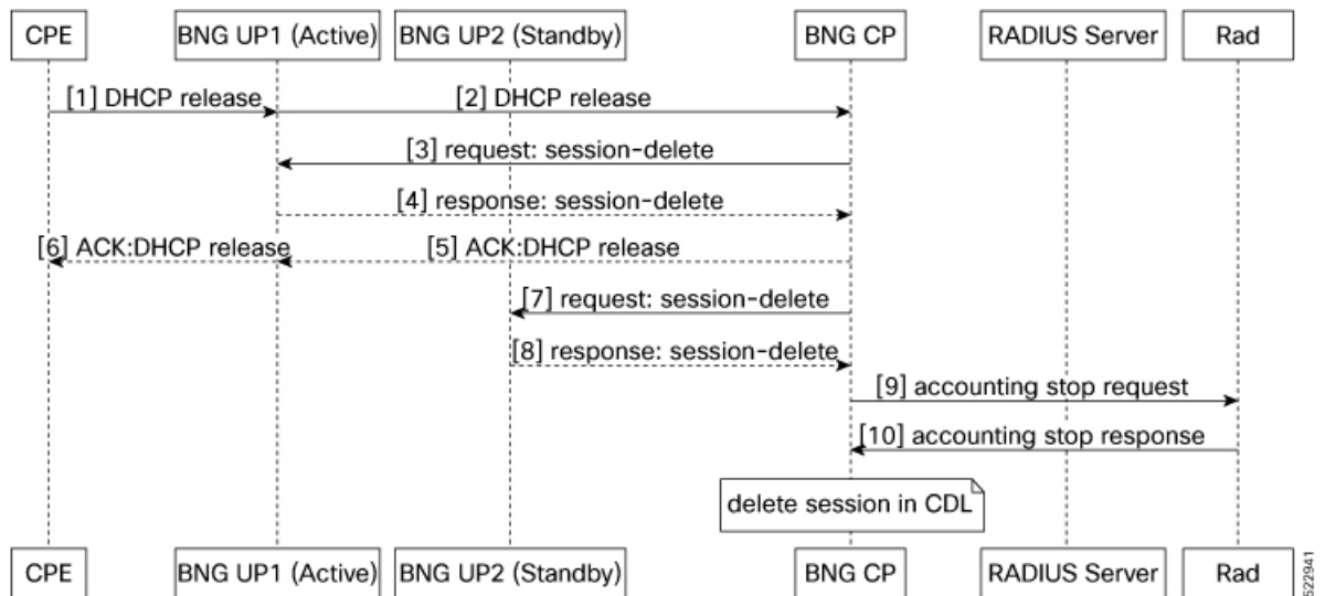
Figure 12: Subscriber Session Deletion Call flow for SRG
