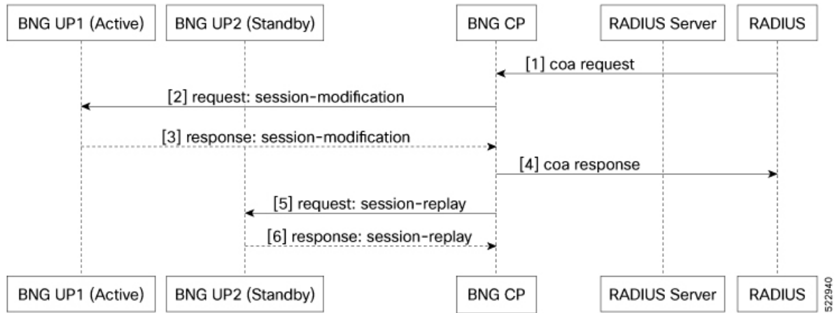
Figure 11: Subscriber Session attributes Modification for SRG
