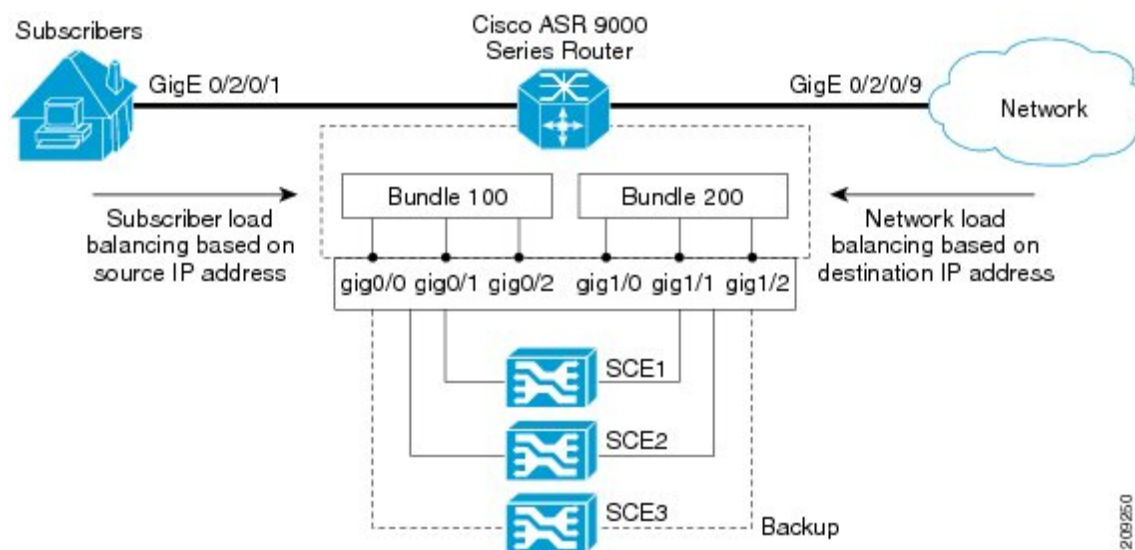
Figure 29: Cisco ASR 9000 Series Router as Dispatcher for SCE Cluster
