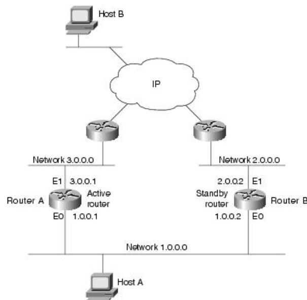
Figure 16: Routers Configured as an HSRP Group
