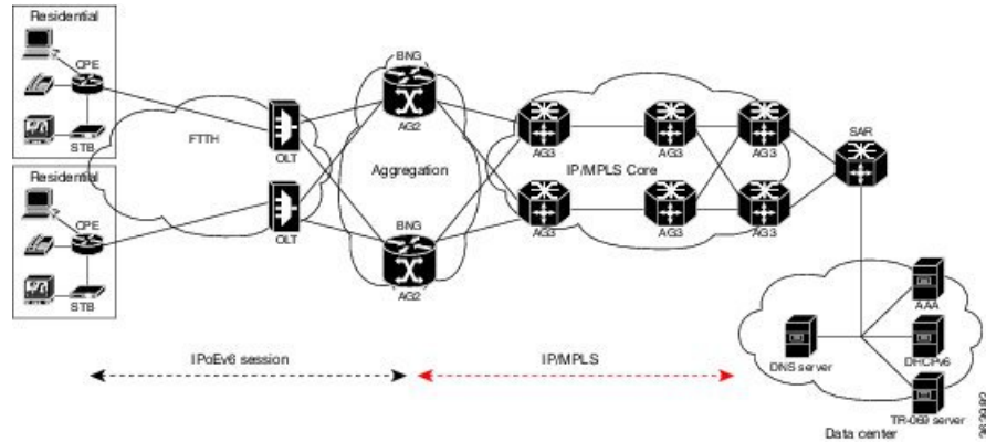
Figure 49: Sample Deployment Topology for Routed Subscriber Sessions
