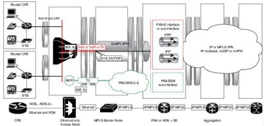
Figure 35: N:1 deployment model for residential subscribers on PWHE
