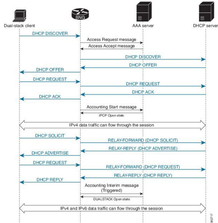
Figure 45: Call Flow of IPoE Dual-Stack - IPv4 Address-Family Starts First
