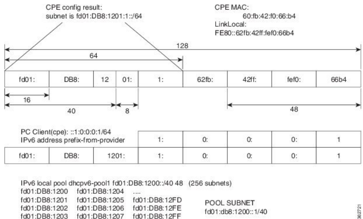
Figure 41: Sample IPv6 Address Mapping for Dual-Stack Subscriber
