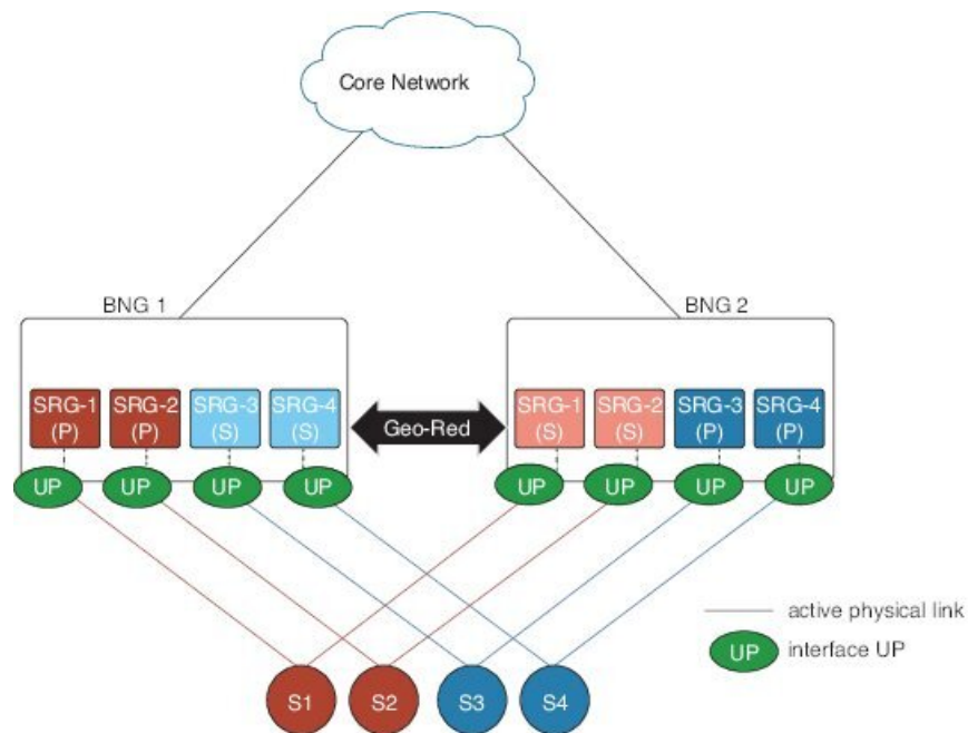
Figure 26: Active-active Session for BNG Geo Redundancy
