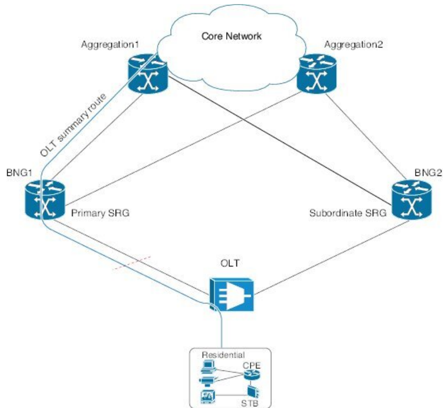
Figure 27: State Control Route for BNG Geo Redundancy
