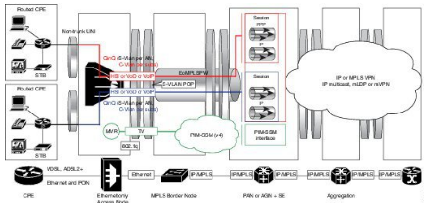
Figure 36: 1:1 deployment model for residential subscribers on PWHE
