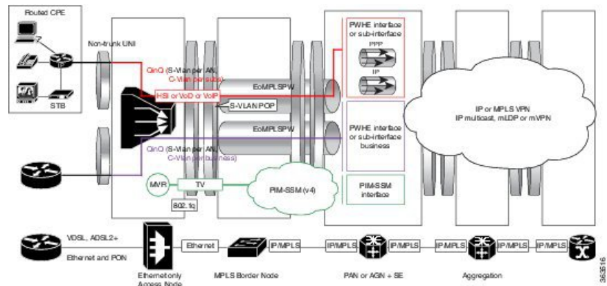
Figure 38: Deployment Model 2 for Residential and Business Subscribers on PWHE
