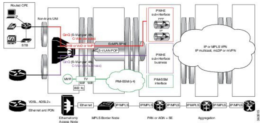
Figure 37: Deployment Model 1 for Residential and Business Subscribers on PWHE
