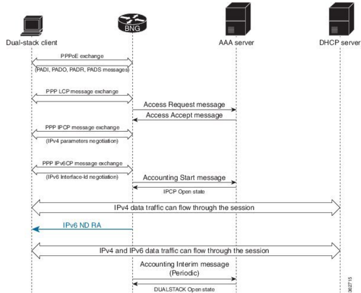
Figure 43: PPPoE Dual-Stack - SLAAC-Based Address Assignment
