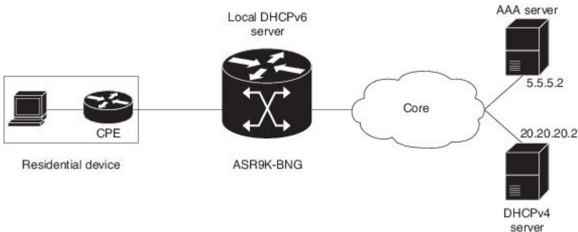
Figure 47: Sample topology for Dual-Stack
