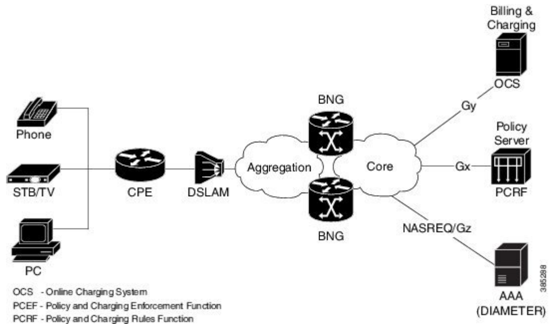
Figure 31: DIAMETER-Geo Redundancy Interworking
