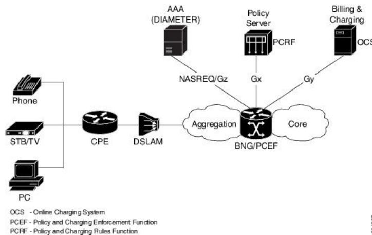
Figure 29: DIAMETER Interface in BNG
