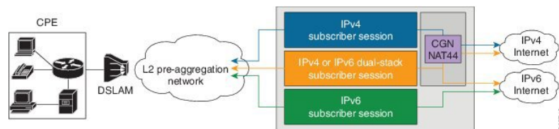
Figure 39: Deployment Model of Dual-Stack Subscriber Sessions
