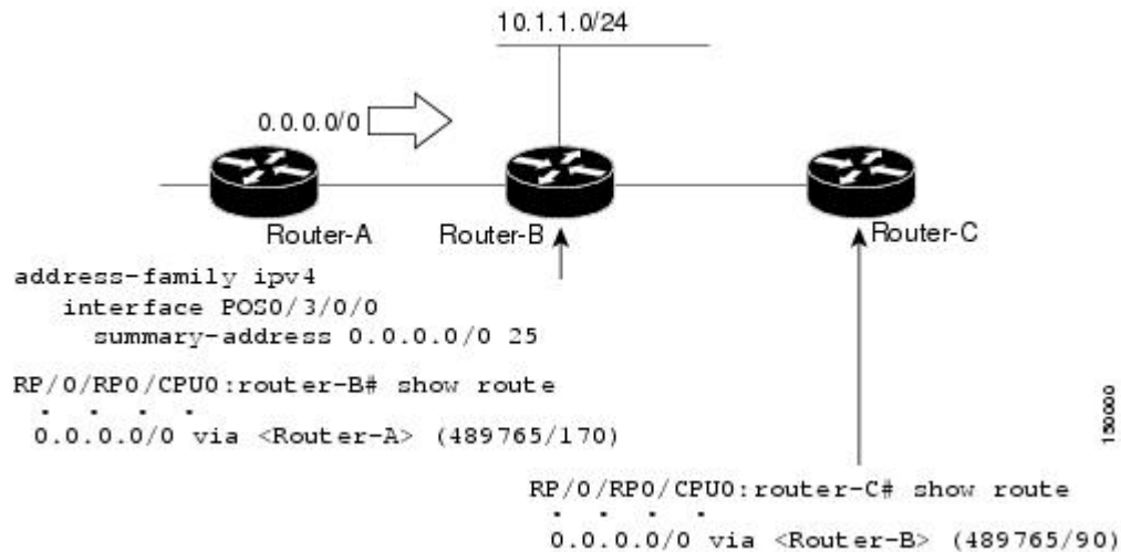
Figure 17: Floating Summary Route Is Applied to Router-B
