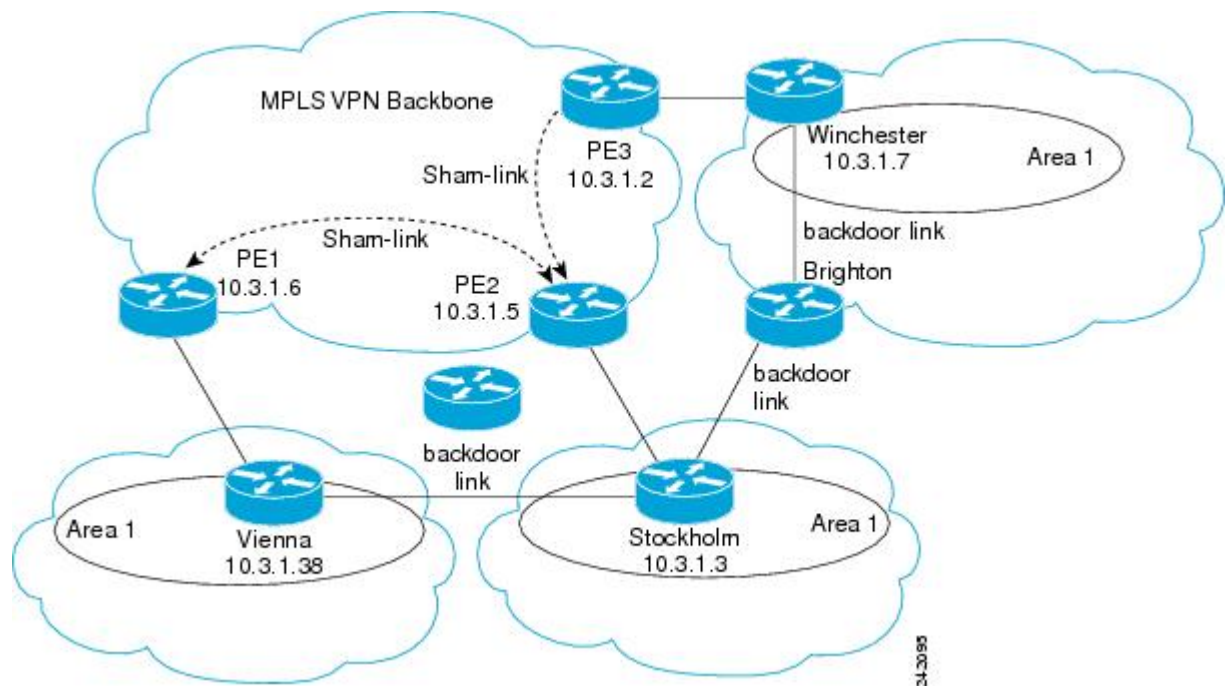
Figure 24: Sham Link Between PE Routers to Connected OSPF Client Sites
