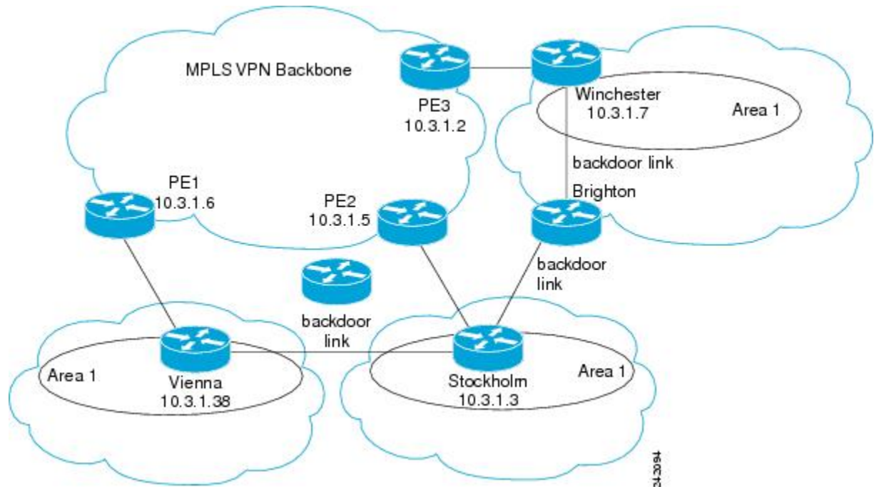
Figure 23: Backdoor Paths Between OSPF Client Sites
