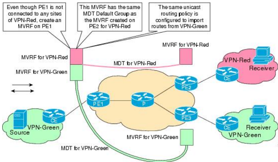
Figure 12: Topology for MVPN Extranet Support Configuration Option 1
