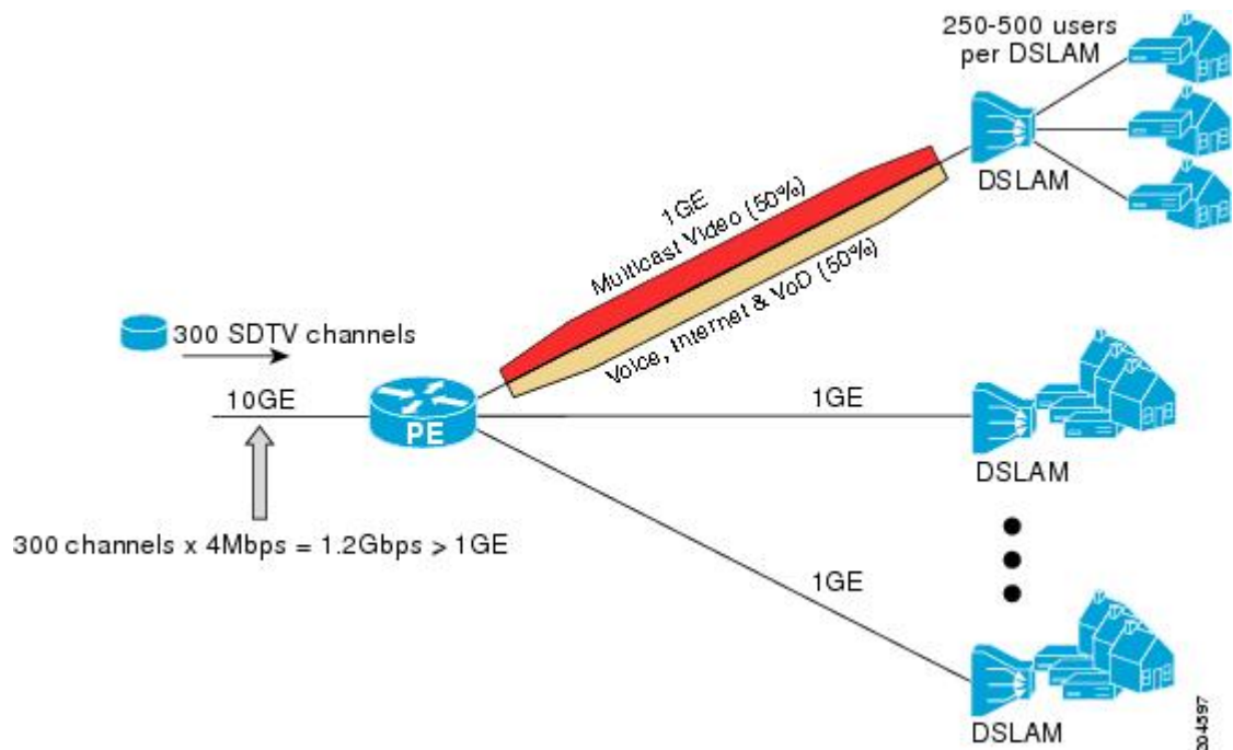
Figure 3: IGMP State Limit Example Topology
