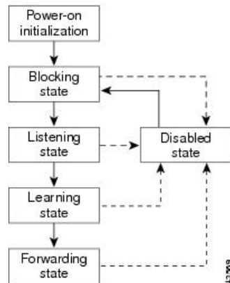
Figure 12: Spanning-Tree Interface States
