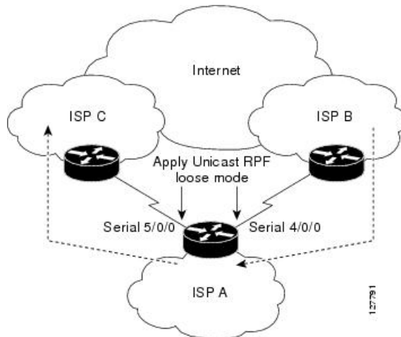
Figure 5: Unicast RPF Loose Mode
