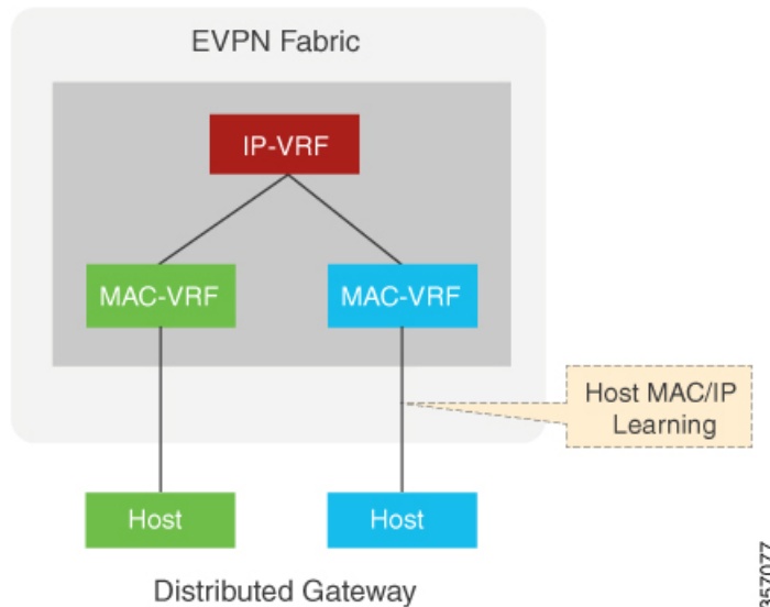
Figure 29: Host MAC-IP Binding on a Single-Homed DAG
