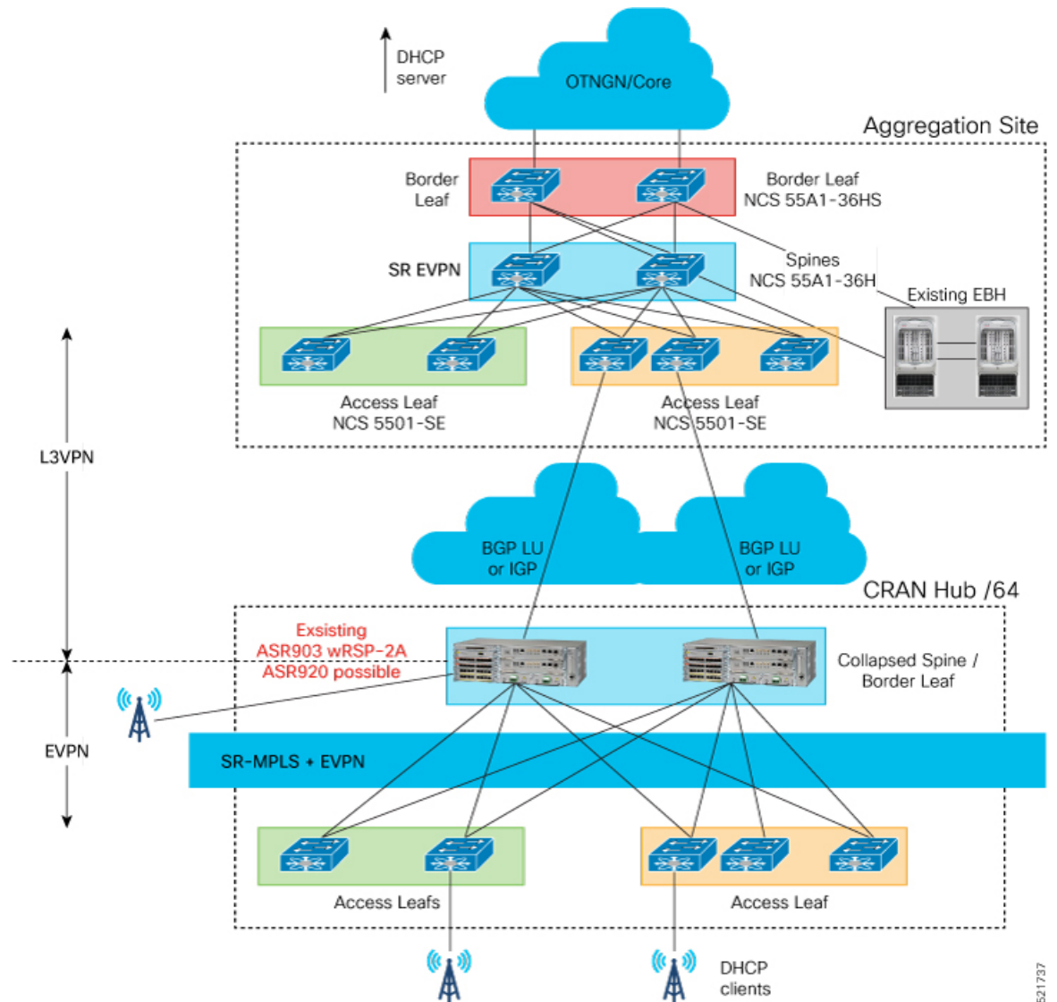
Figure 31: DHCP Relay Agent Network Topology
