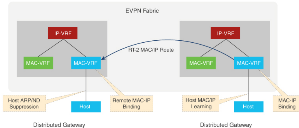
Figure 30: ARP and ND Flooding Suppression
