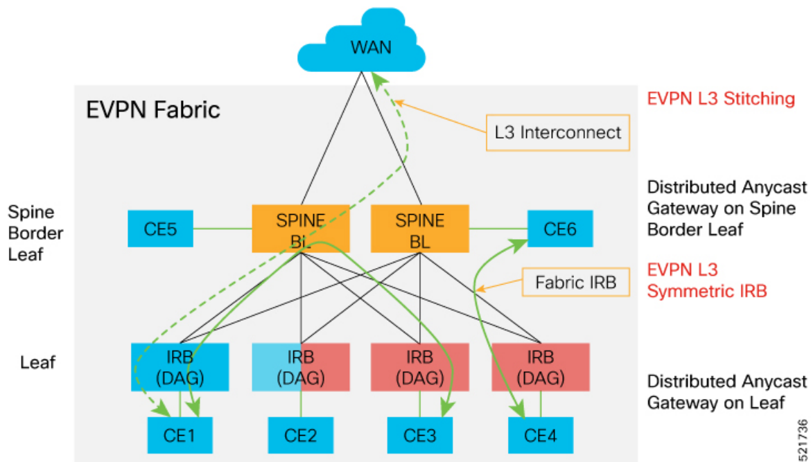
Figure 33: Collapsed Spine or Leaf or RR on a Single Node Network Topology
