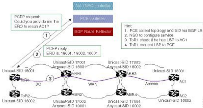
Figure 8: ODN Operation
