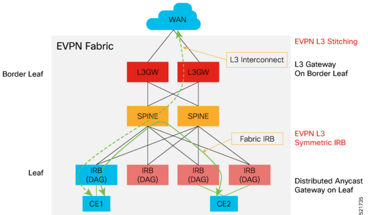
Figure 32: Single Homing DAGs with Symmetric IRB Network Topology
