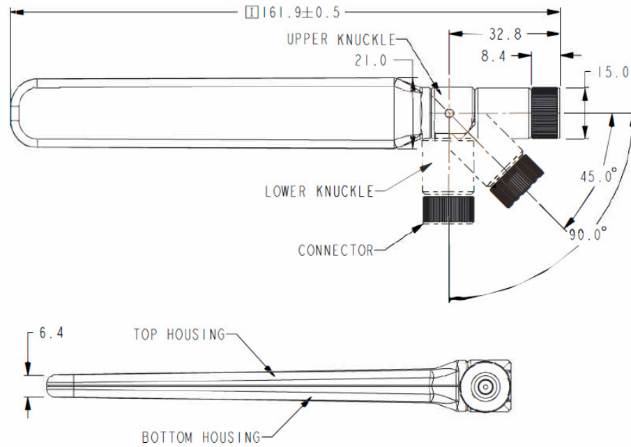
Figure 2: Mechanical Drawing
