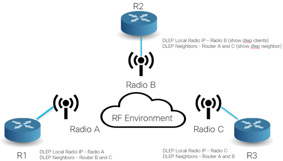
Figure 5: Show DLEP Configuration
