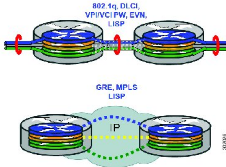
Figure 181: Path Level Virtualization
