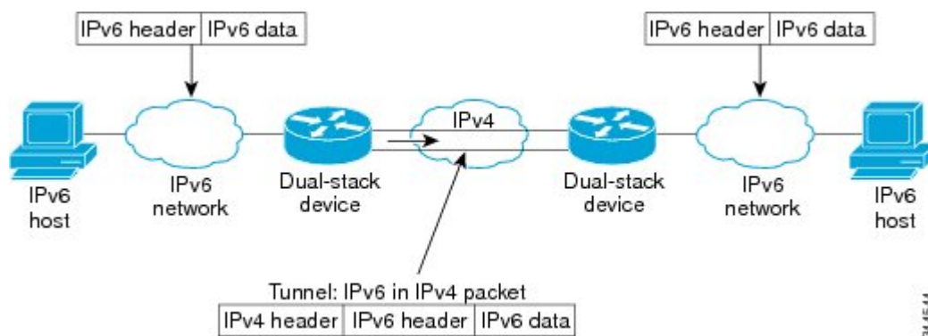
Figure 216: Overlay Tunnels
