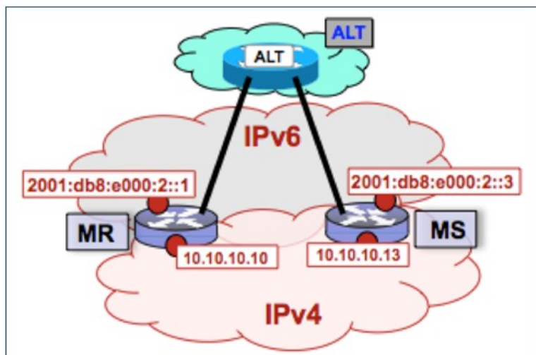
Figure 160: ALT-Connected LISP Map Resolver and Map Server, each having both an IPv4 and an IPv6 RLOC
