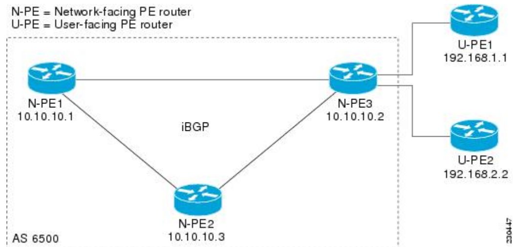
Figure 95: Network Diagram for VPLS Autodiscovery Using BGP and the L2VPN Address Family
