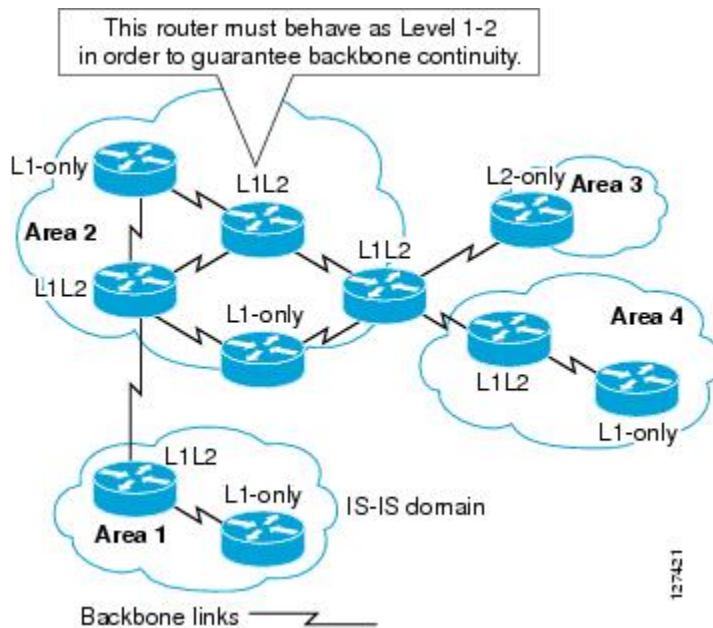
Figure 141: Level 1, Level 2, and Level 1-2 Devices in an IS-IS Network Topology
