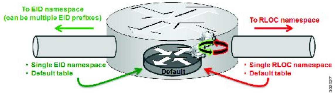
Figure 182: Default (Non-Virtualized) LISP Model (Resolves Both EID and RLOC Addresses in the Default (Global) Routing Table).
