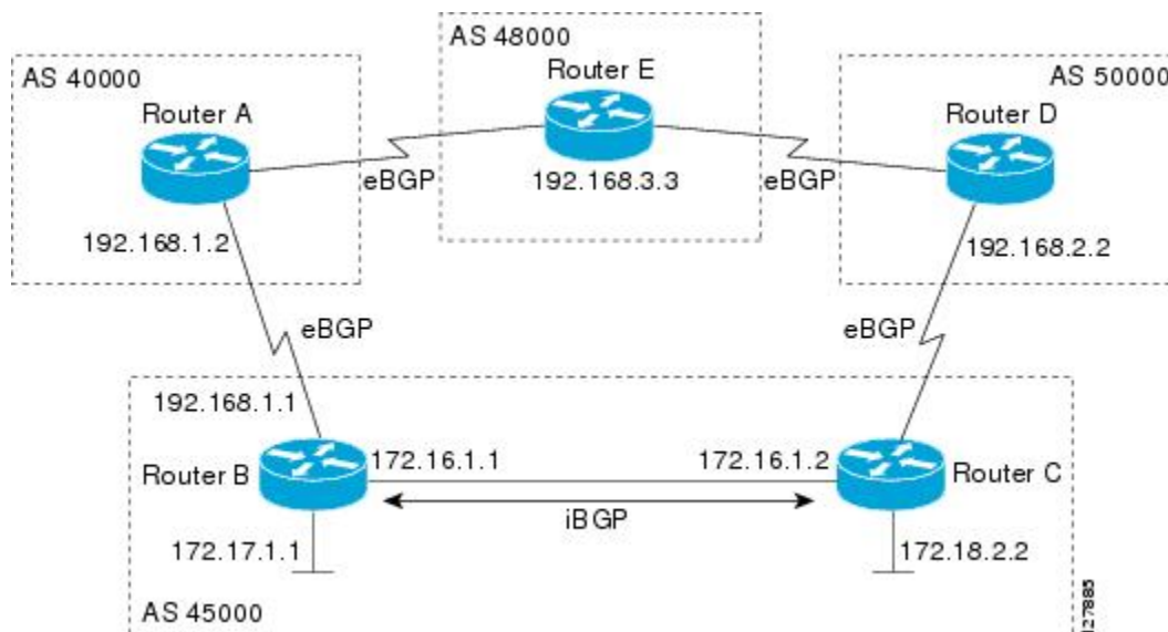
Figure 57: Network Topology for Outbound Path Selection
