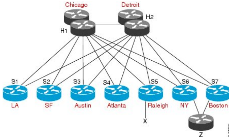
Figure 119: DMVPN Deployment
