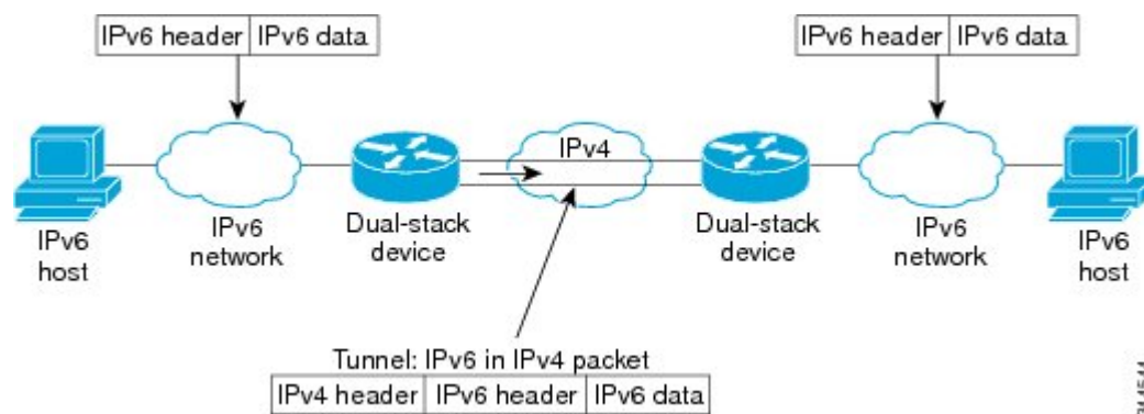
Figure 213: Overlay Tunnels
