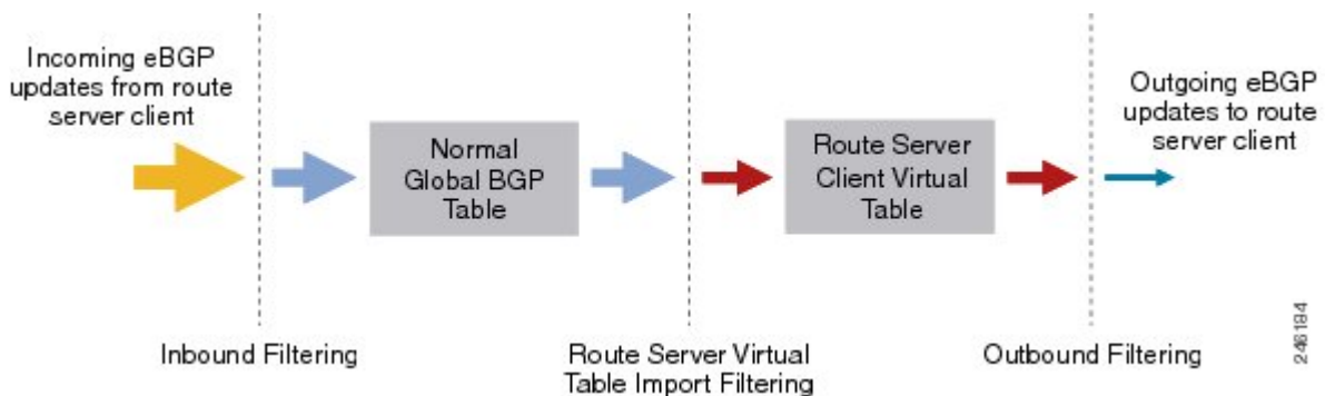
Figure 112: Route Server Filtering in Three Stages
