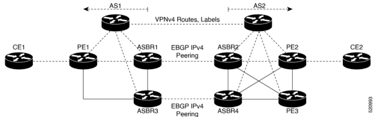
Figure 98: MPLS VPN Inter-AS Option C Deployment
