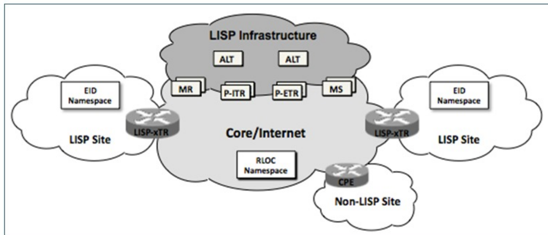
Figure 1: Cisco IOS XE LISP Deployment Environment
