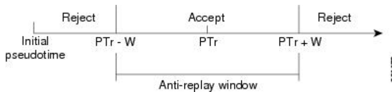
Figure 137: Antireplay Window
