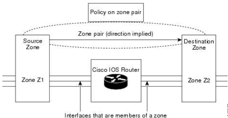
Figure 52: Zone Pairs
