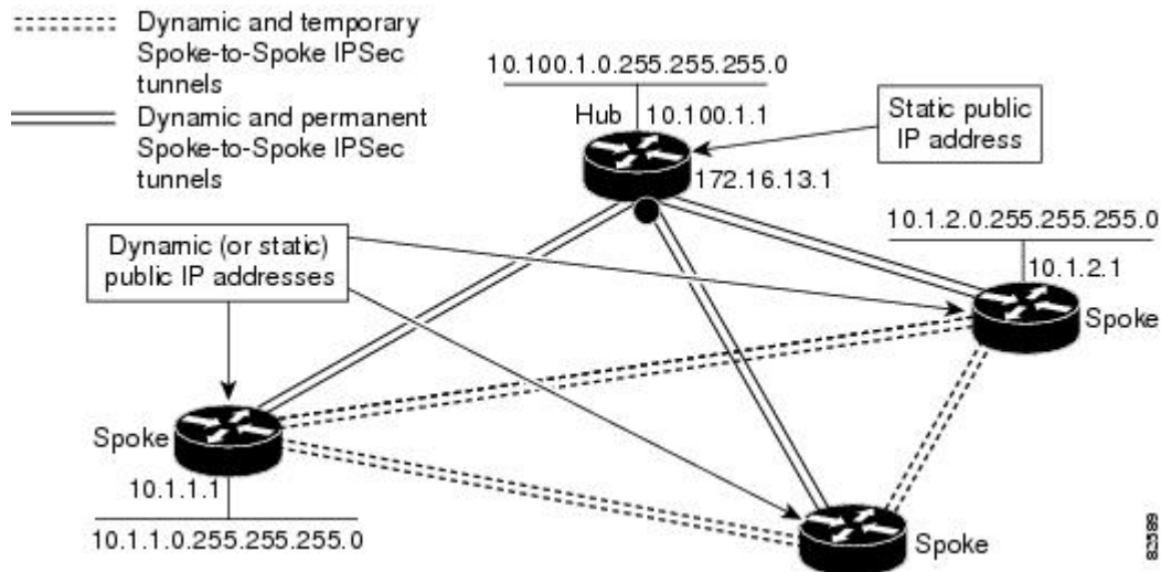
Figure 103: Sample mGRE and IPsec Integration Topology
