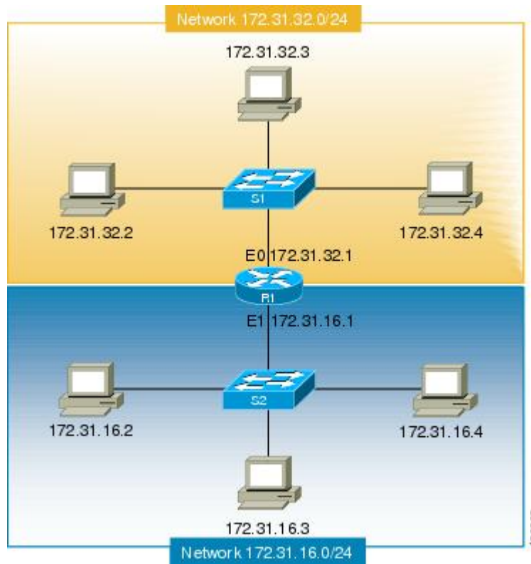
Figure 4: Correctly Configured Network
