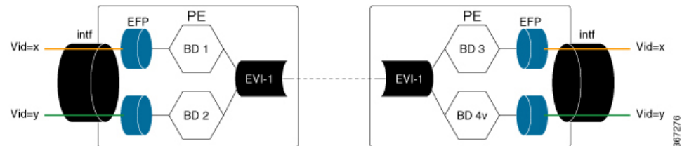
Figure 21: VLAN-Aware Bundle Service Interface
