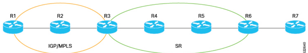
Figure 27: LSR Support for Autoroute Announce SR Policies
