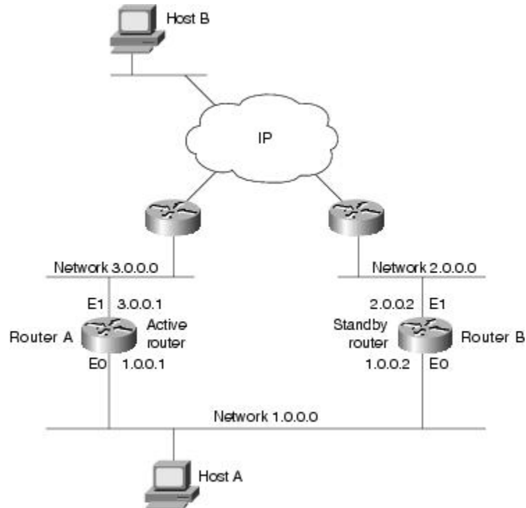
Figure 2: Routers Configured as an HSRP Group
