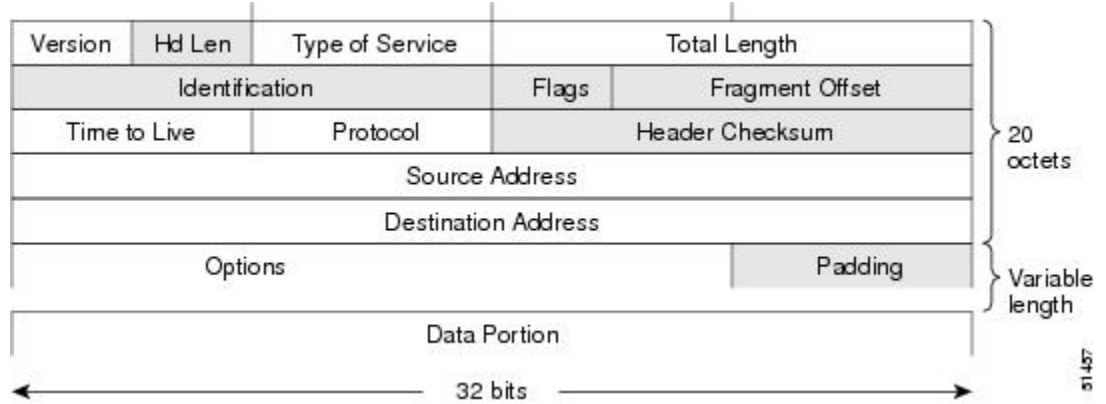
Figure 9: IPv4 Packet Header Format
