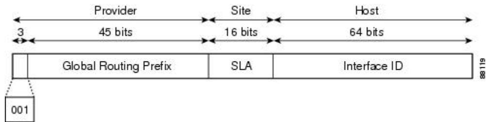
Figure 4: Aggregatable Global Address Format
