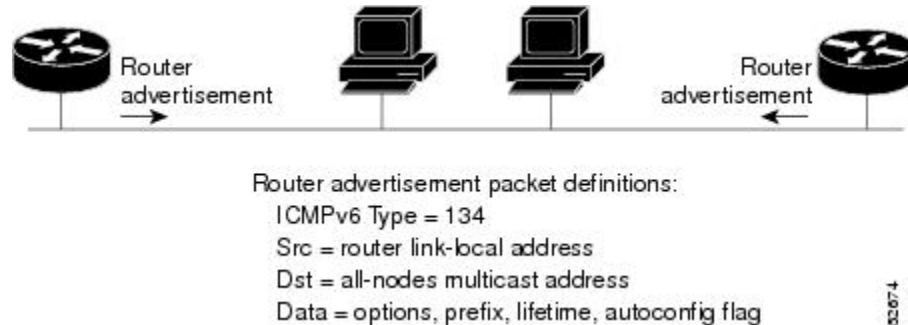
Figure 13: IPv6 Neighbor Discovery—Router Advertisement Message
