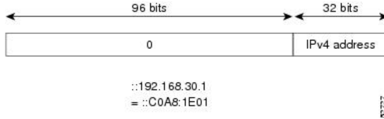
Figure 6: IPv4-Compatible IPv6 Address Format
