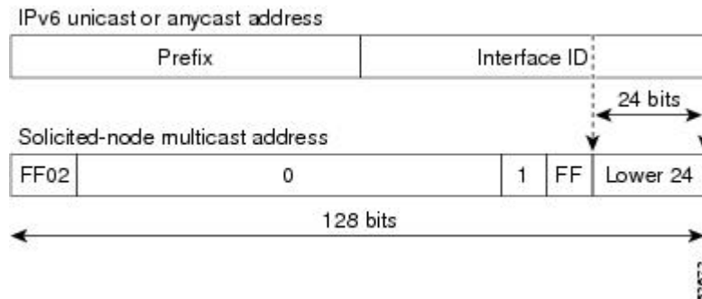
Figure 8: IPv6 Solicited-Node Multicast Address Format
