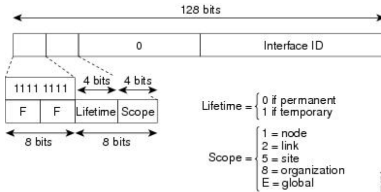
Figure 7: IPv6 Multicast Address Format
