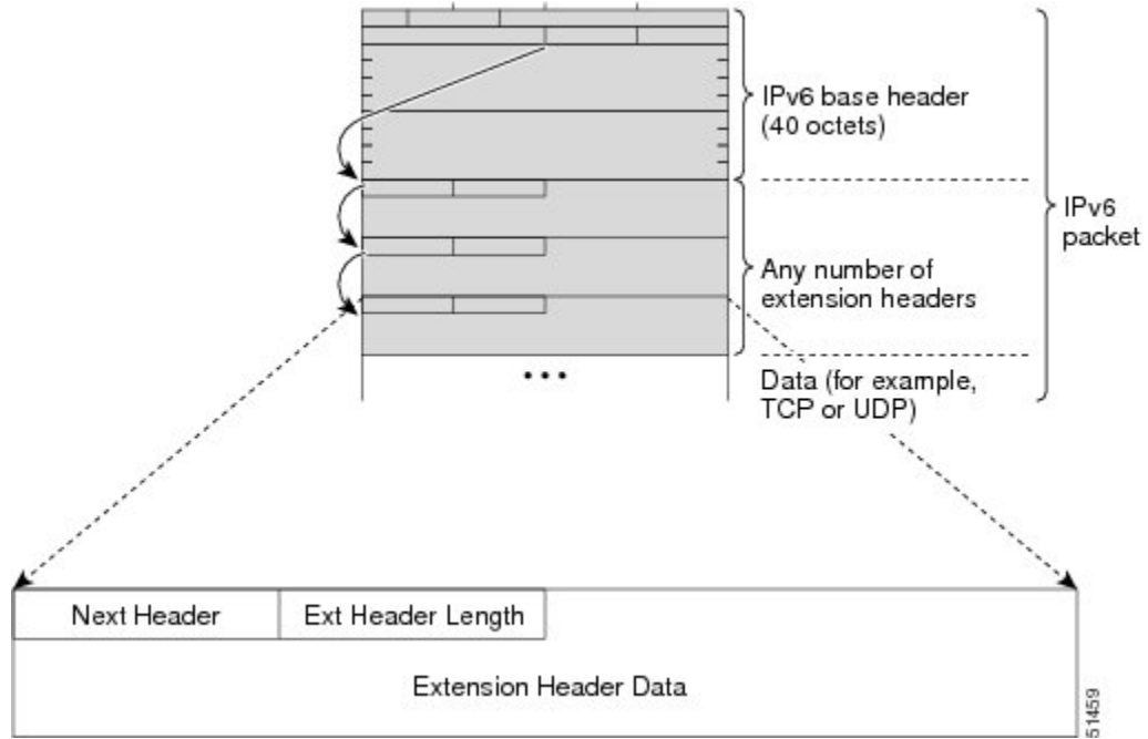
Figure 11: IPv6 Extension Header Format
