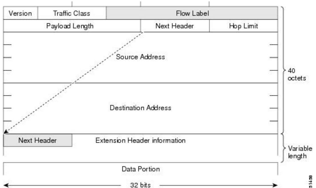
Figure 10: IPv6 Packet Header Format
