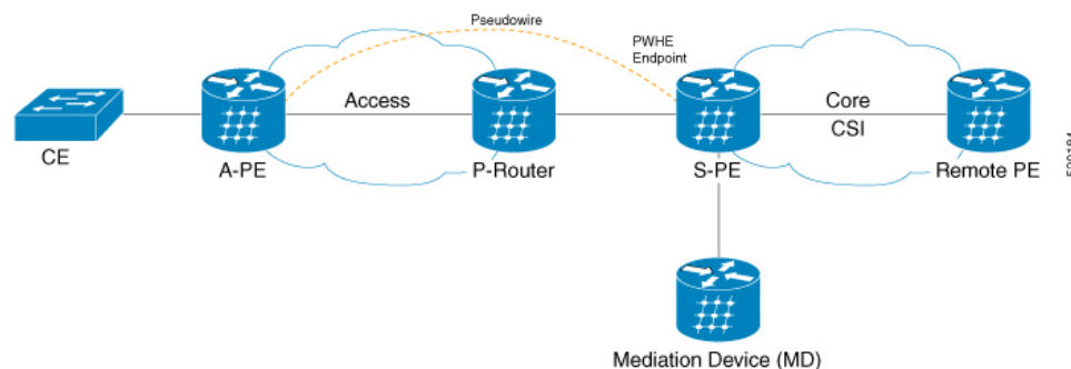
Figure 9: Lawful Intercept
